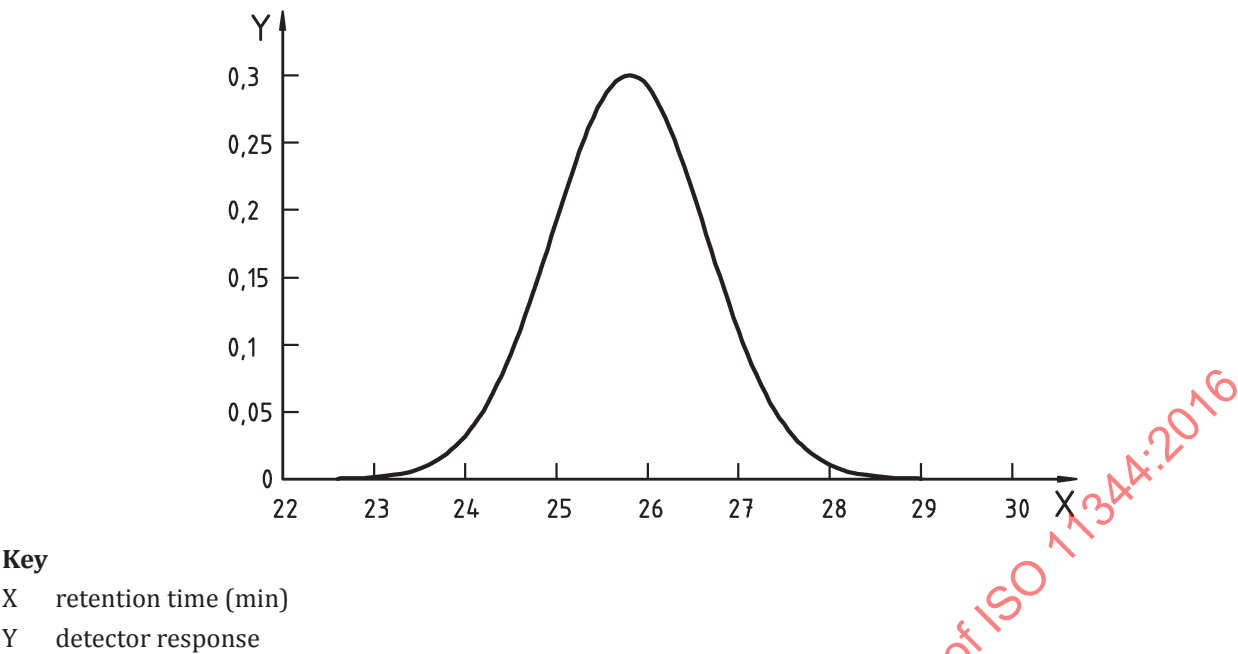
Figure A.1 — GPC chromatogram acquisition
