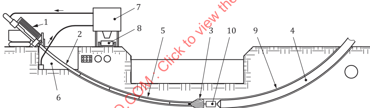
Figure 22 — Schematic representation of replacement by horizontal directional drilling — Pilot bore
