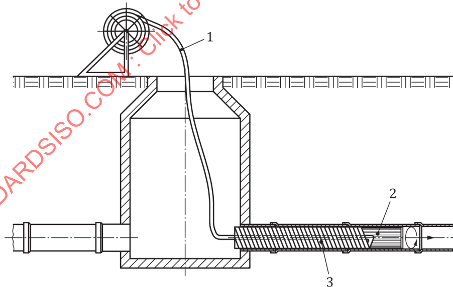
Figure 12 — Lining with spirally-wound pipes — Schematic representation of expanded liner winding from the manhole (Method A2)
