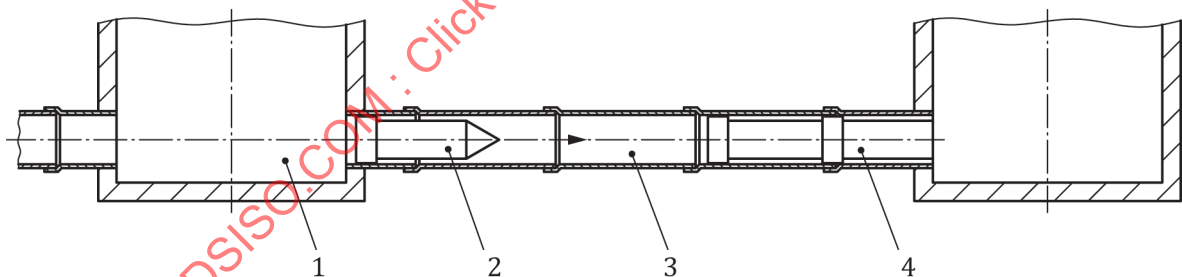
Figure 8 — Lining with discrete pipes — Schematic representation of installation by pulling (Method B)
