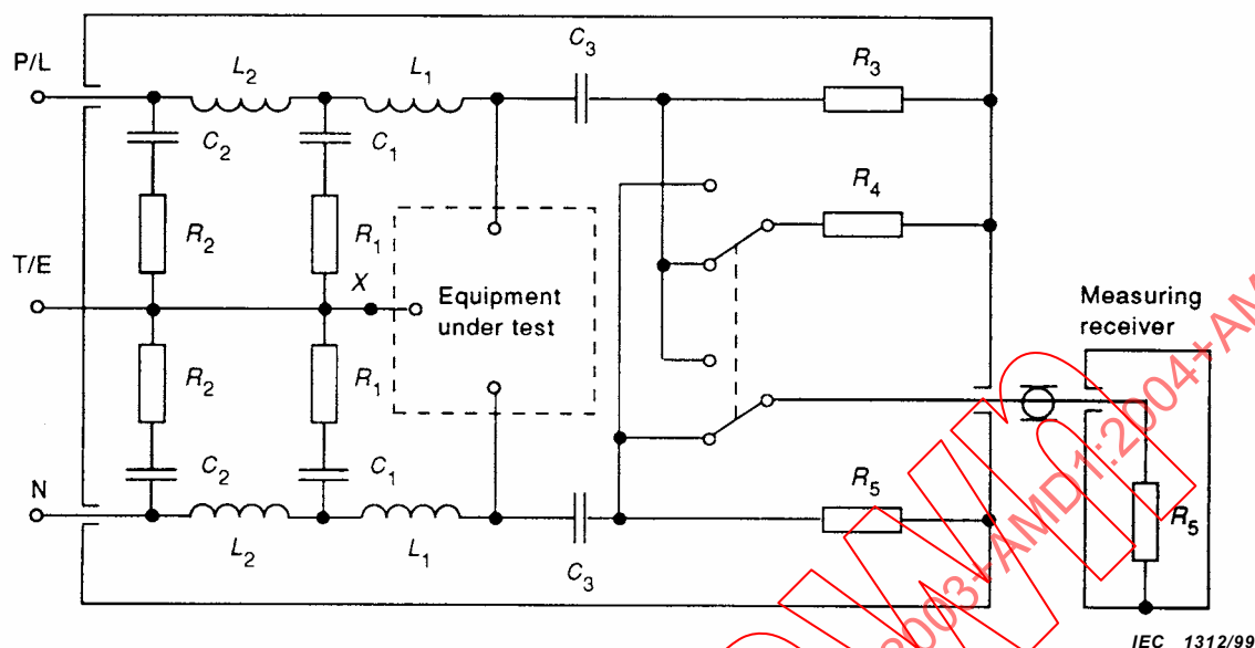
Figure 4 – Example of artificial mains 50 \Omega/50 \mu\text{H} + 5 \Omega V-network (see 4.2 and clause A.2)
