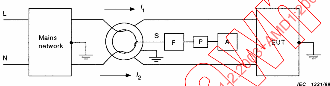
Figure B.4b – Test circuit which differentiates common (asymmetrical mode and differential (symmetrical) mode noise
