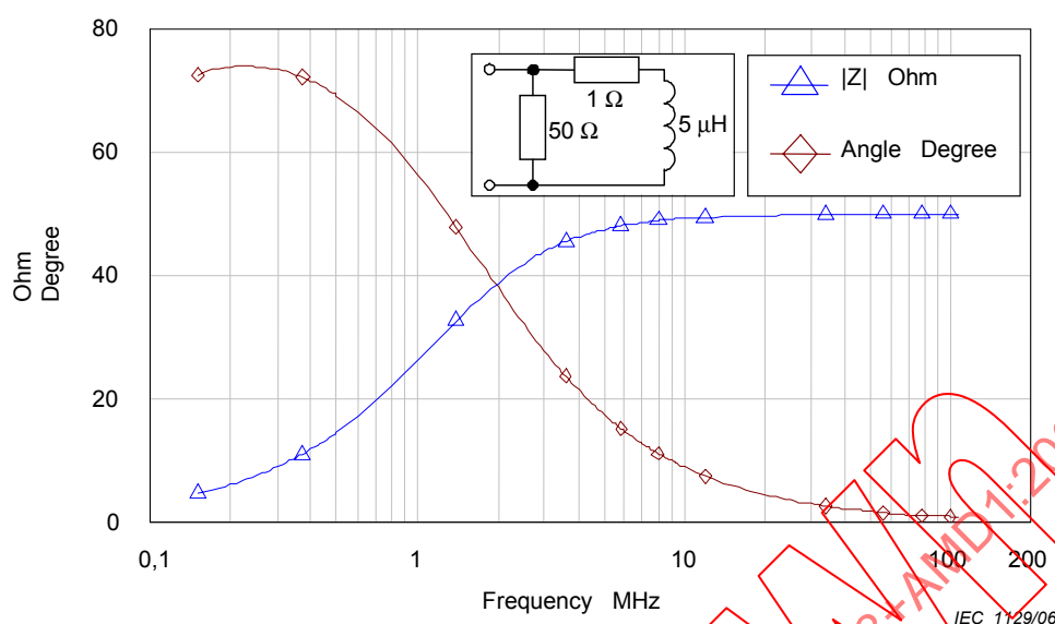
Figure 2 – Impedance (magnitude and phase) of the V-network for bands B and C (from 0,15 MHz to 108 MHz; see 4.4)
