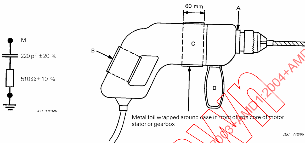
Figure 9a – RC element
