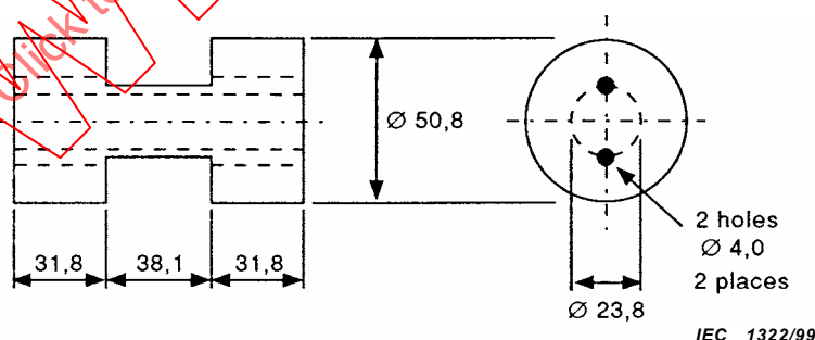
Figure B.5 – Shield configuration used with current transformer (The material should be highly conductive, e.g. copper or brass)
