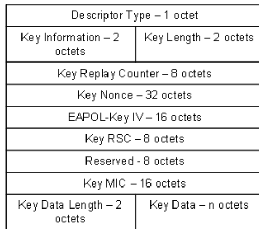
Figure 43u—EAPOL-Key frame
