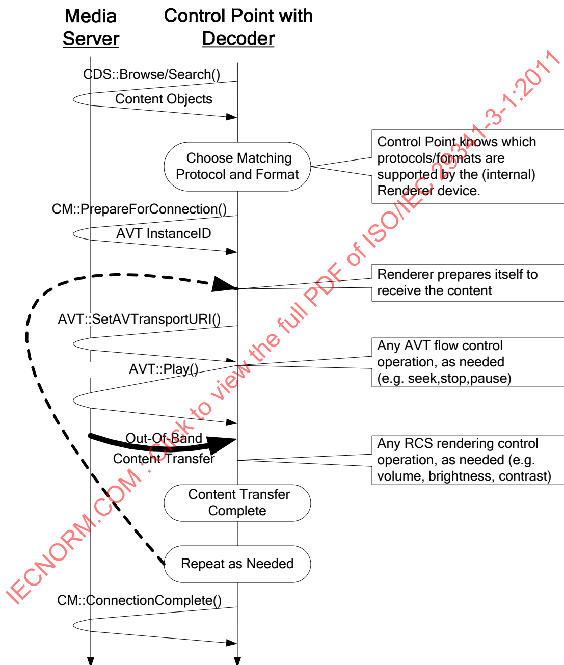
Figure 9 — 2-Box model: Control Point with Decoder using Isochronous-Push
