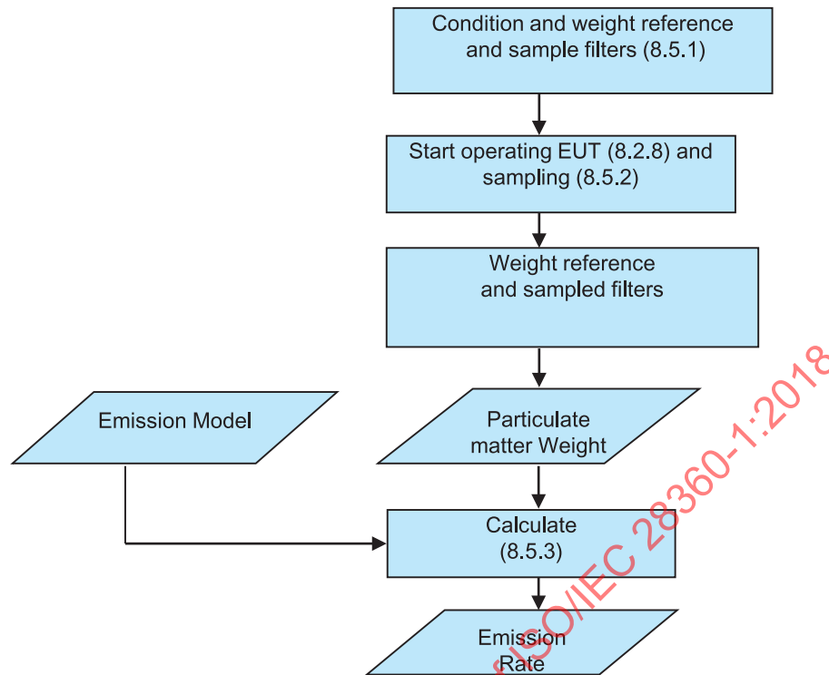
Figure 4 — Determination method for particulate matter
