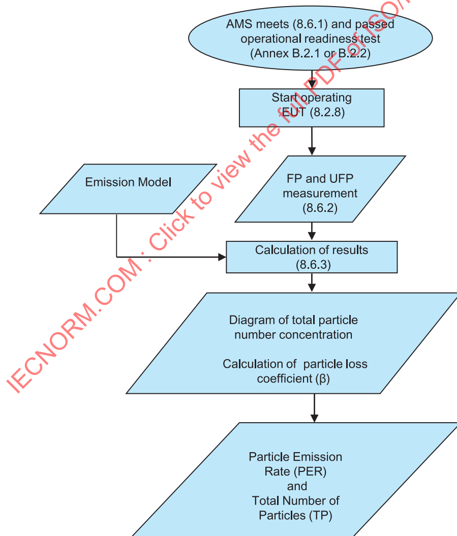
Figure 5 — Determination method for FP and UFP emissions
