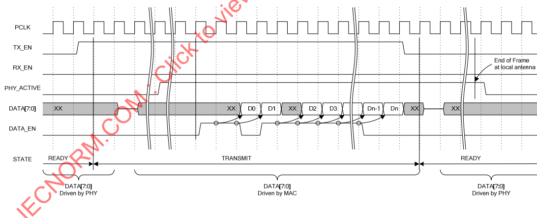
Figure 19 – Single Frame Transmit Timing
