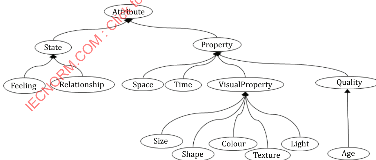
Figure 6 — Subclasses of jponto:Attribute
