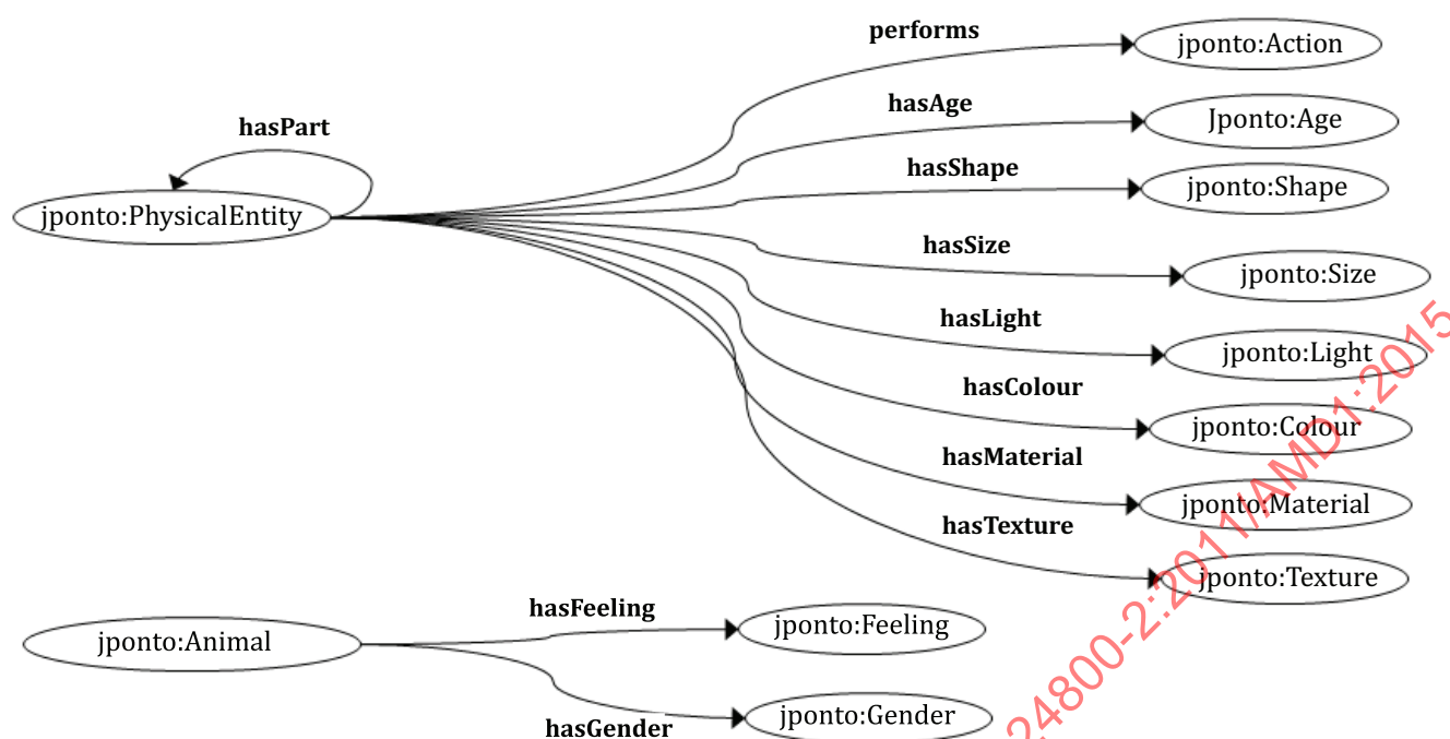
Figure 8 — Specific properties of JPonto-visual (arrows show the domain and range of the property)
