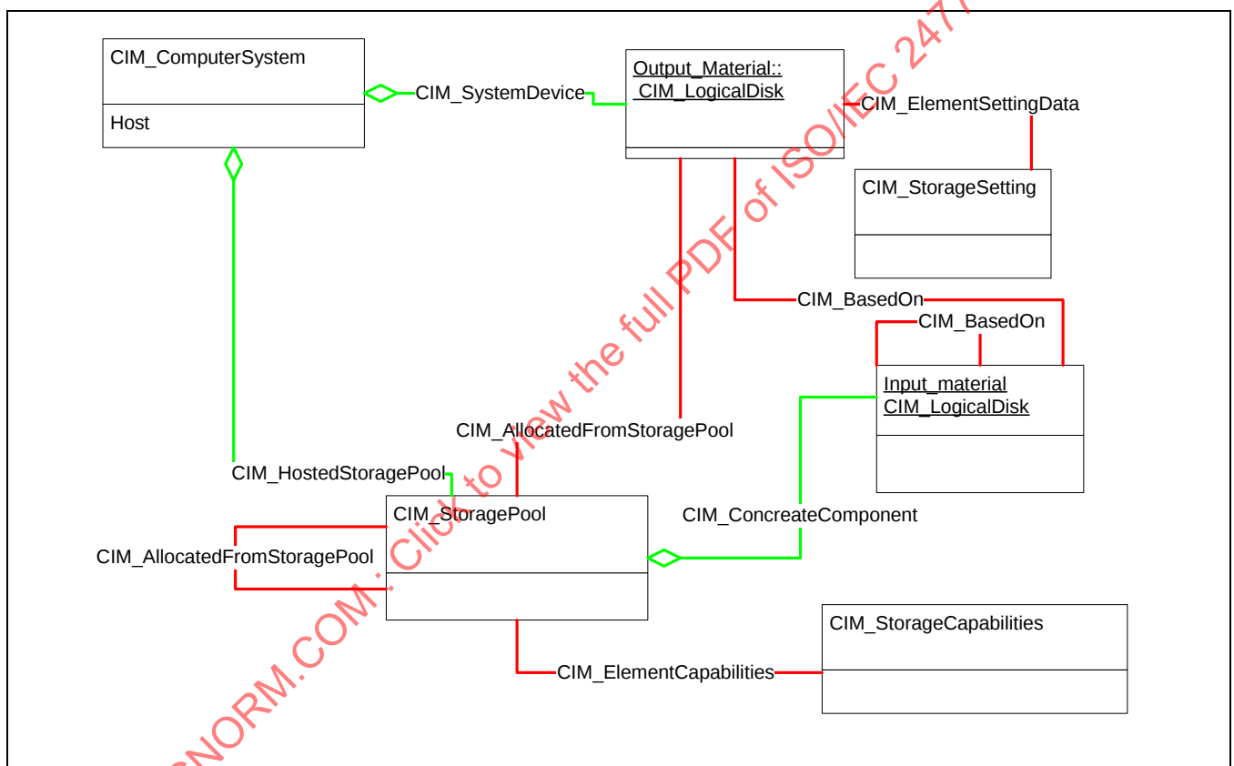
Figure 123 - Volume Management Instance Diagram
