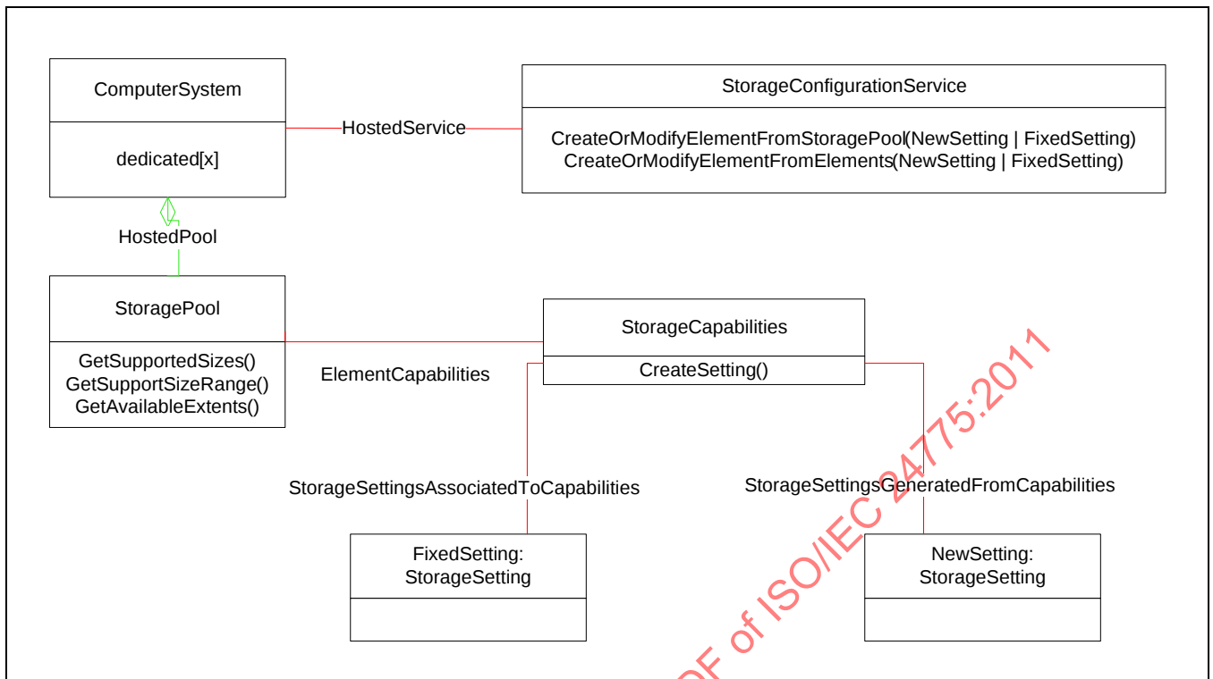
Figure 156 - Volume Creation - Step 2
