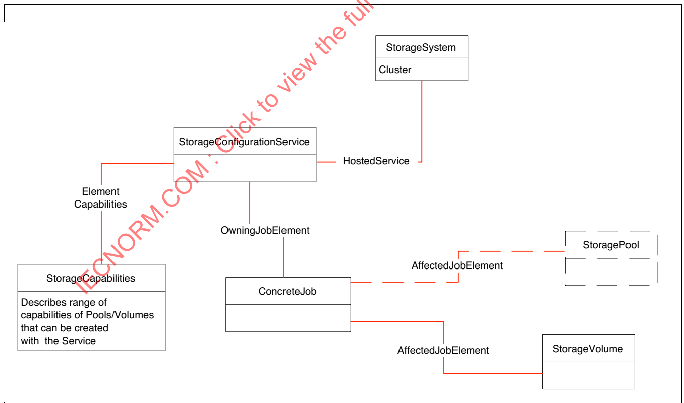
Figure 145 - Storage Configuration
