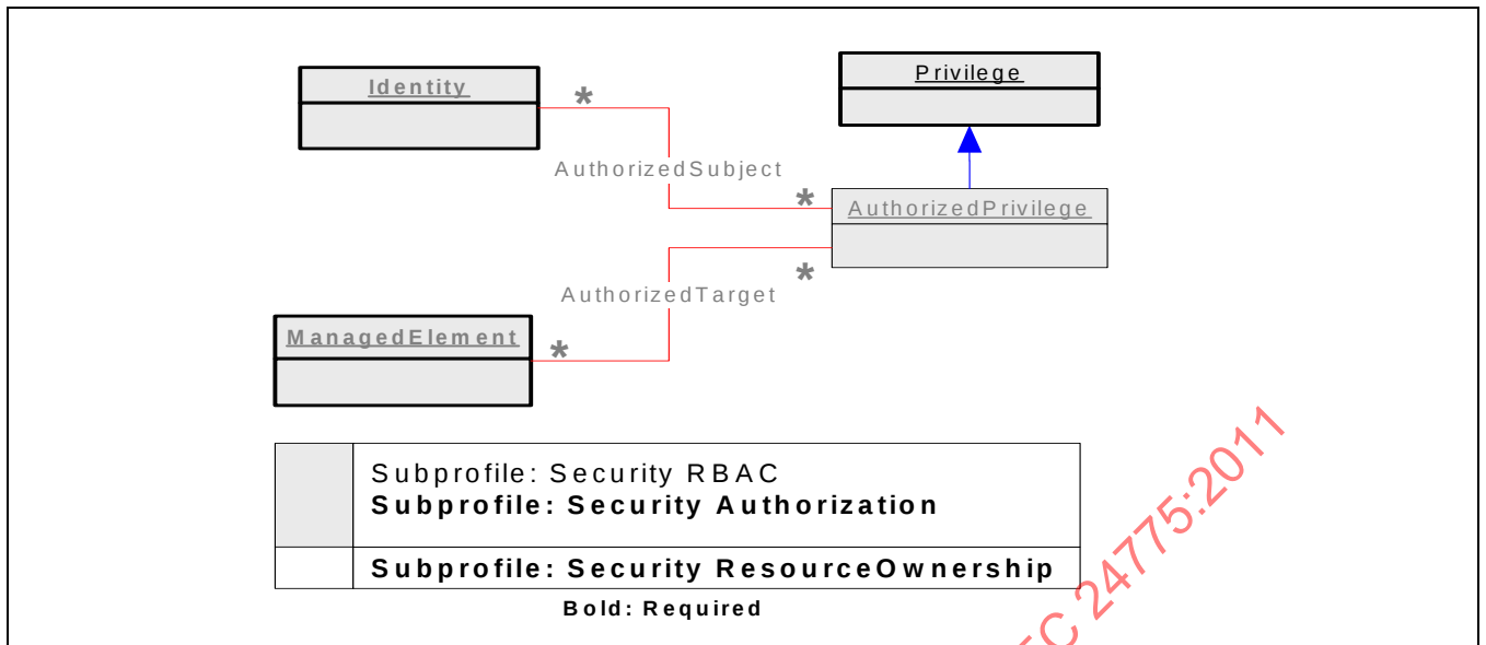
Figure 76 - AuthorizedPrivilege
