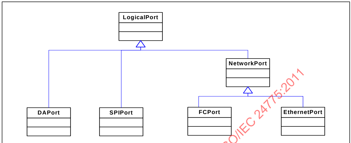
Figure 61 - Logical Port Hierarchy
