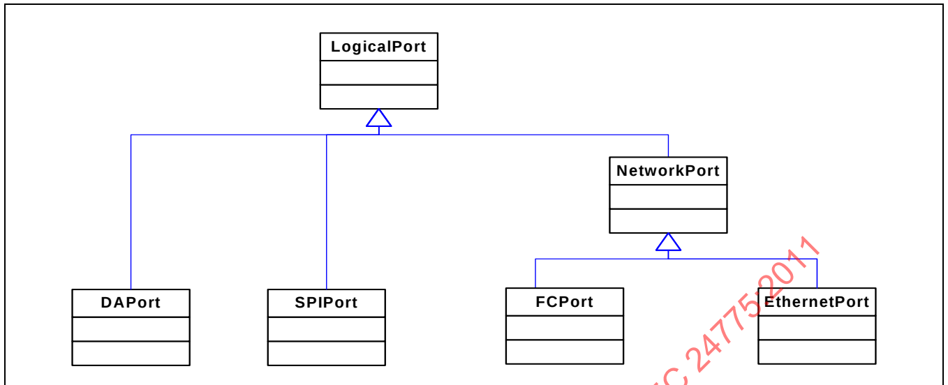
Figure 55 - Port Class Hierarchy
