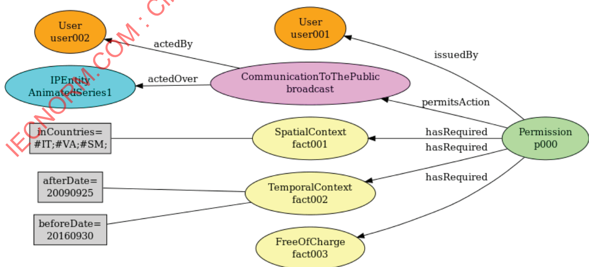
Figure 16 — Expression of a permission, extracted from a real contract
