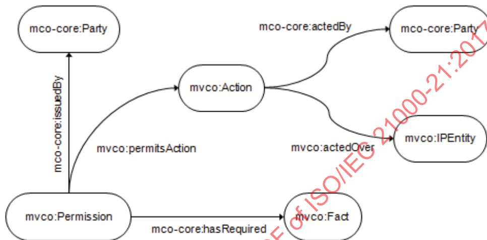
Figure 6 — Classes and object properties around permission
