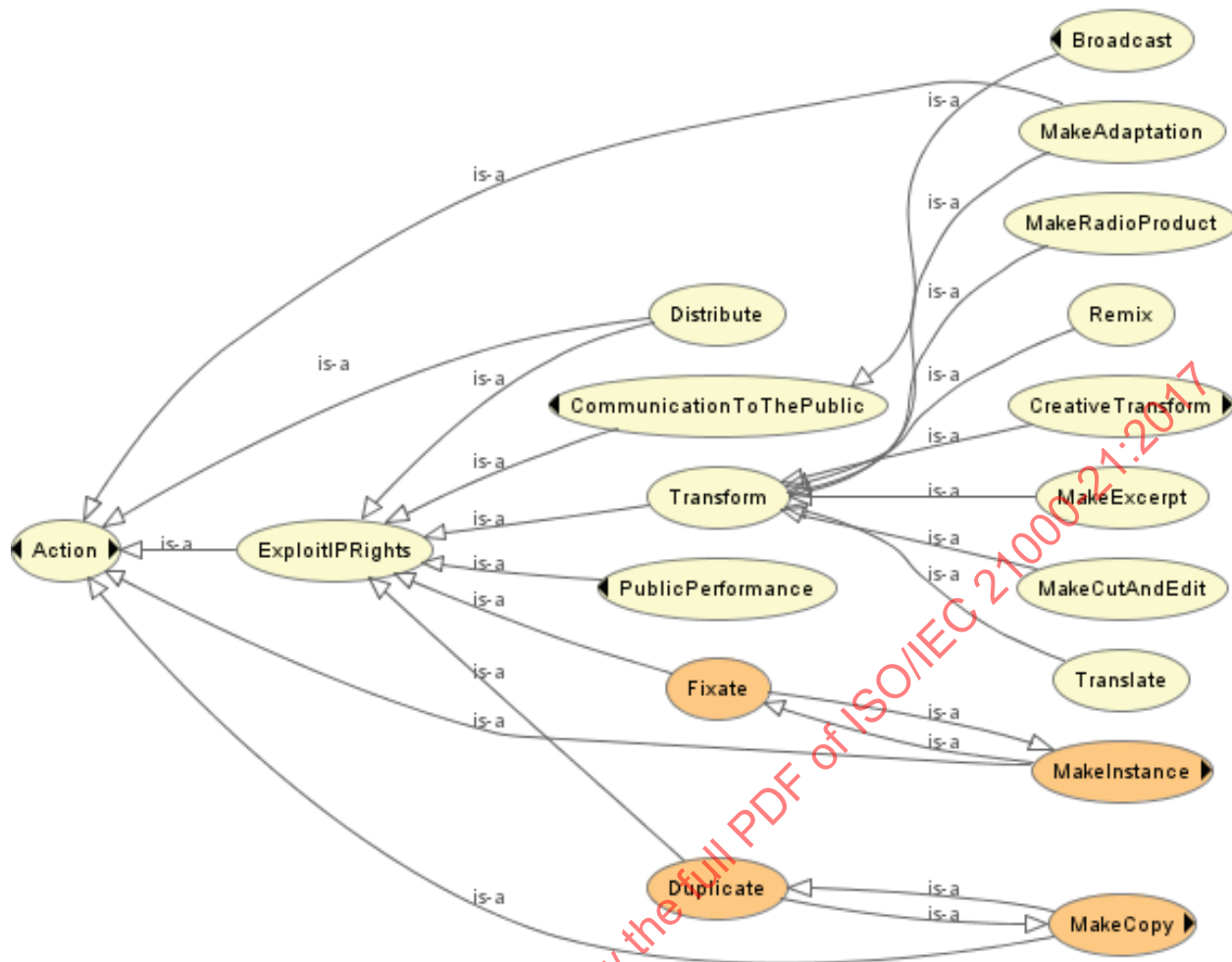
Figure 24 — Subclasses of mco-ipre:ExploitationIPRights inheritance from other mvco:Action
