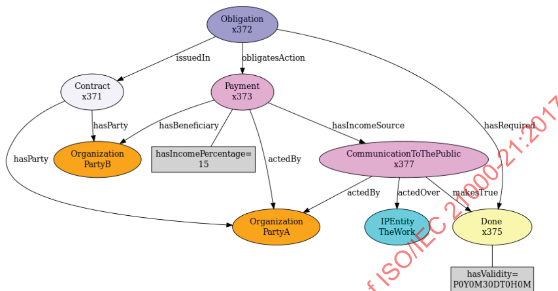
Figure 21 — Example of payment expressed as a percentage of an exploitation income
