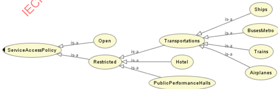
Figure 31 — Subclasses of mco-ipre:ServiceAccessPolicy
