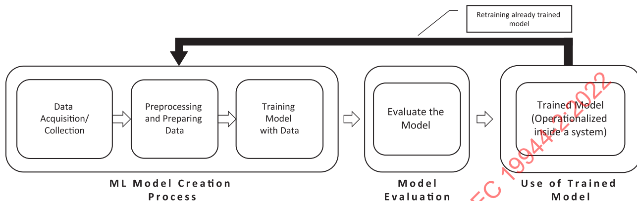
Figure 1 — Example of a data acquisition and processing pipeline for AI
