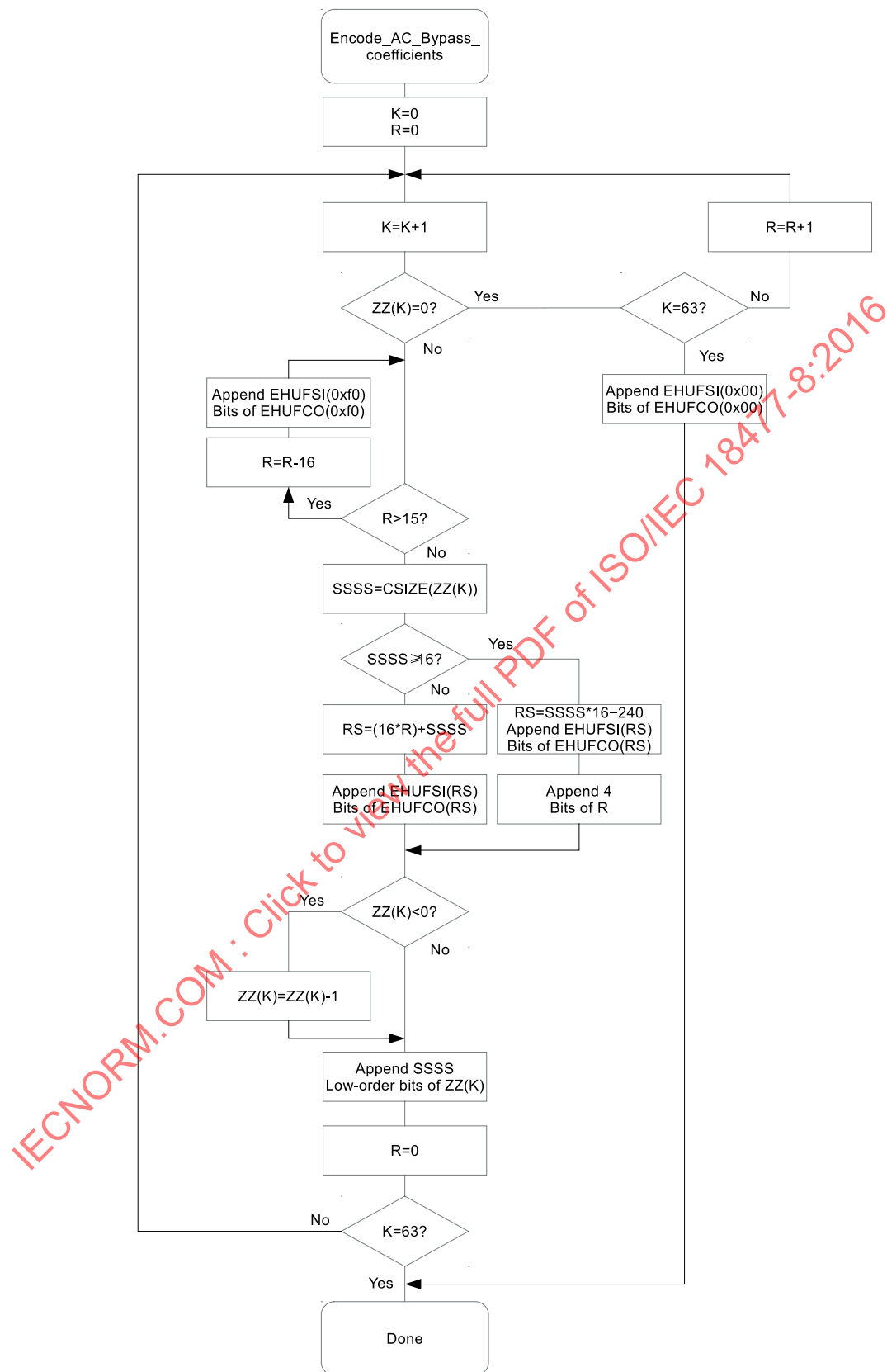
Figure D.3 — Encoding procedure for large-range coding
