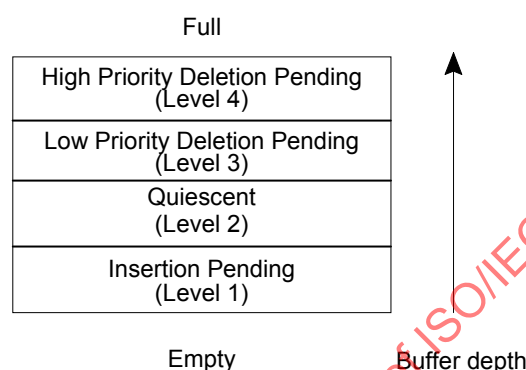
Figure A.2 — Clock skew management states
