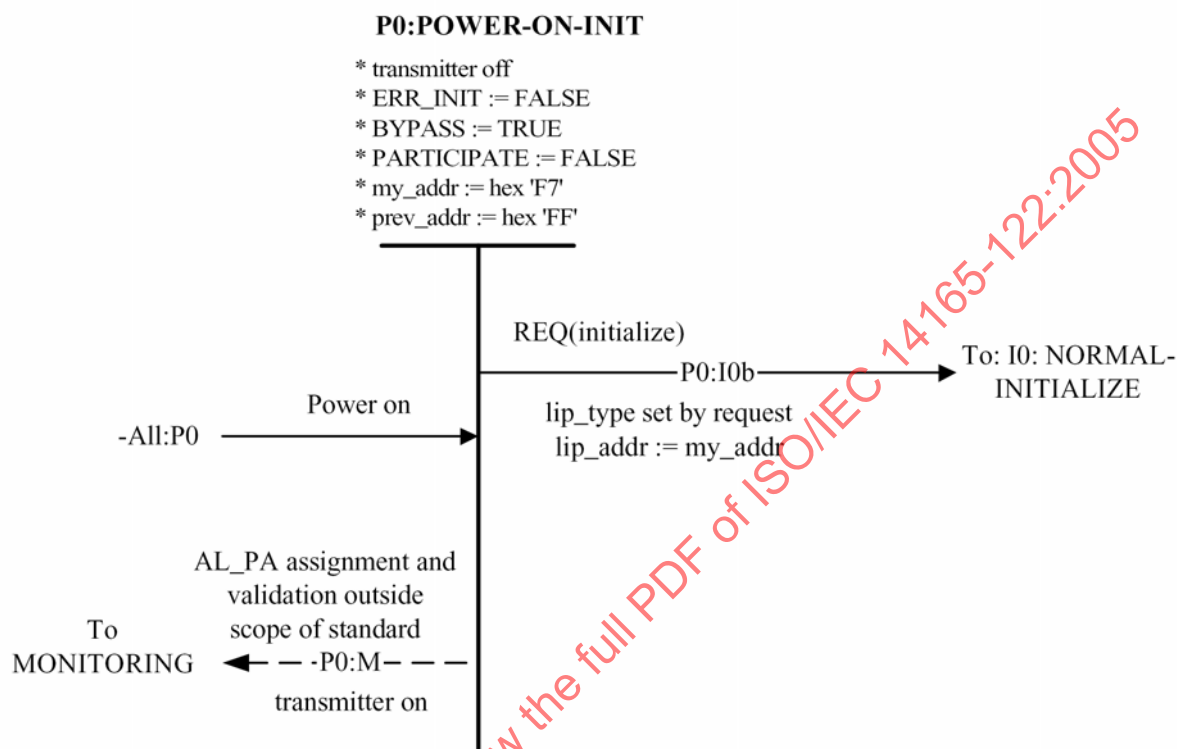
Figure 8 — POWER-ON state diagram
