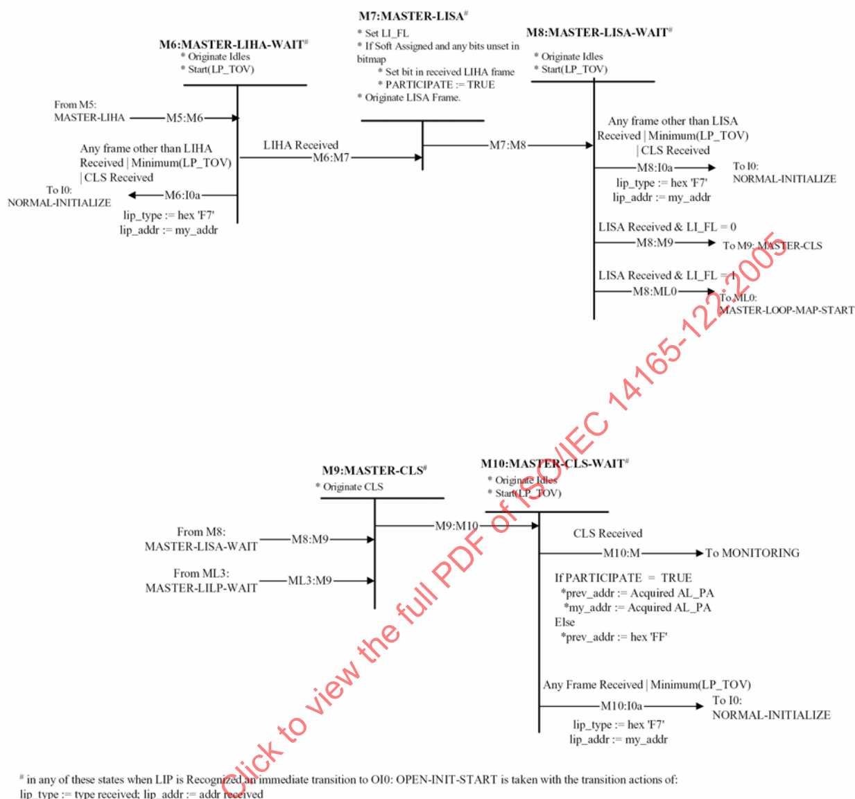
Figure 15 (concluded) — Master Initialization state diagram
