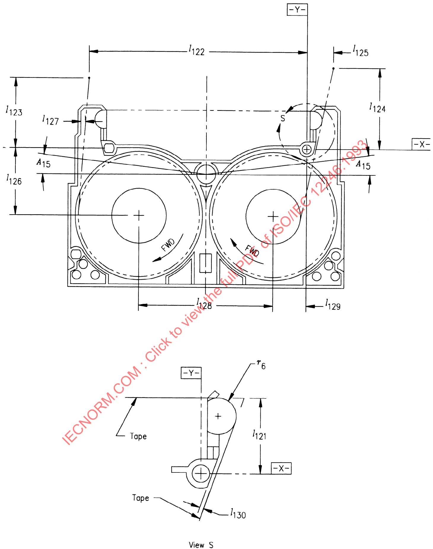
Figure 16 - Internal tape path and light path
