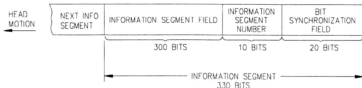
Figure 24 - Information Segment Layout
