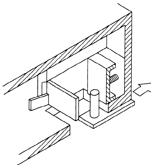
Figure 12 - Direction of force needed to unlock the reel lock
