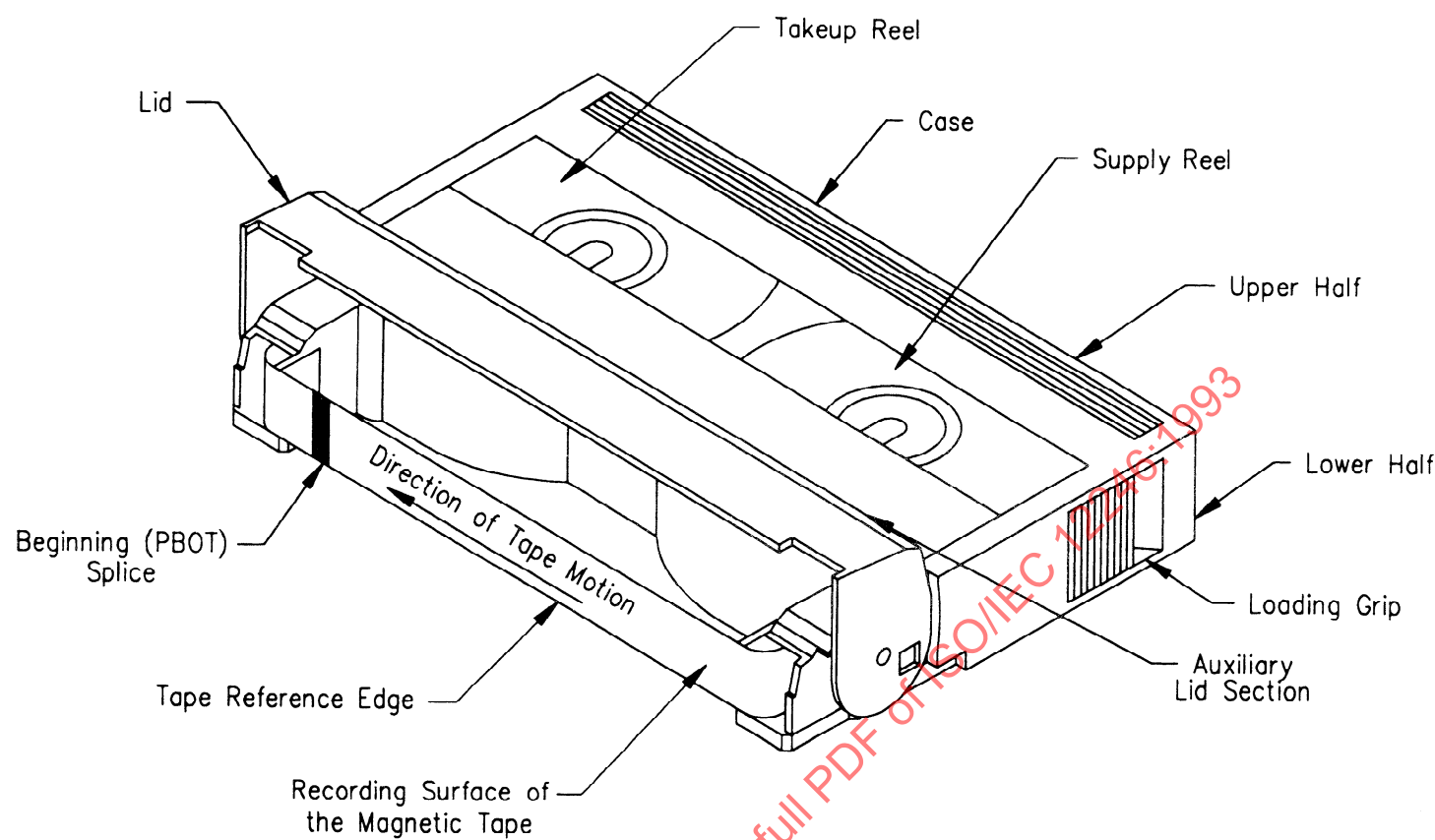
Figure 1 - Tape cartridge assembly top view (lid open)
