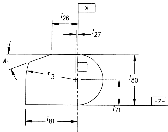
Details of the Side of the Lid
