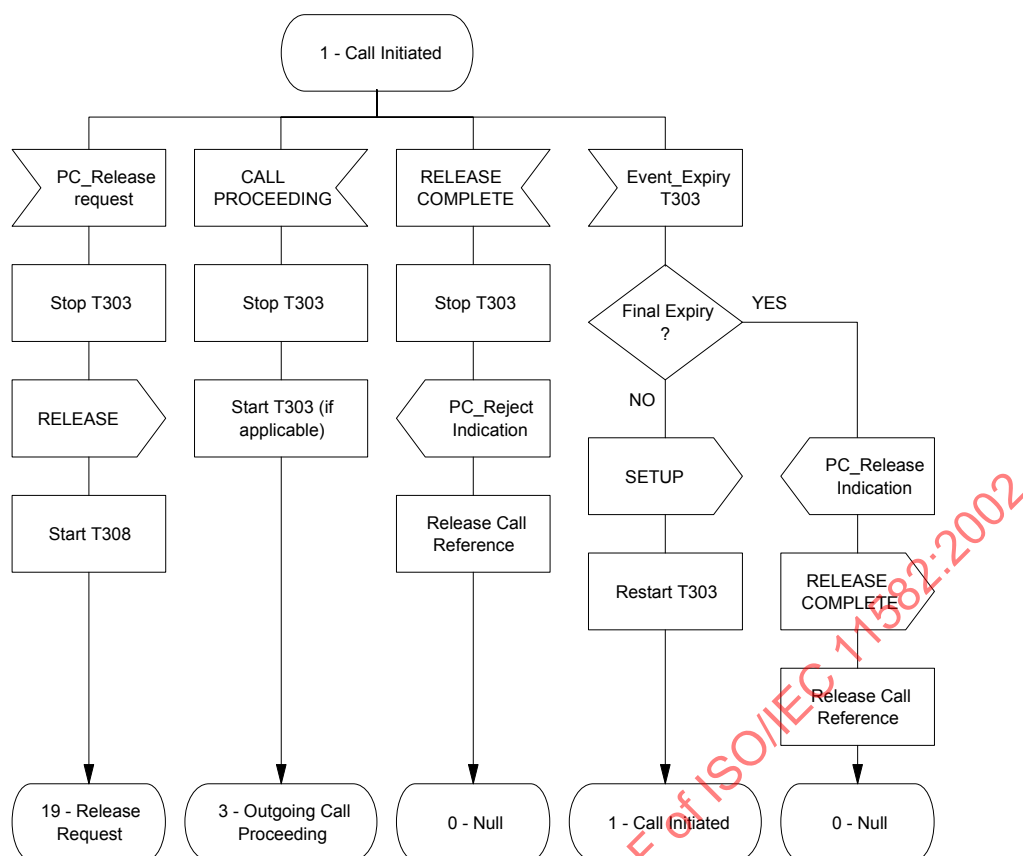
Figure 9 — Connection oriented Protocol Control SDL (Sheet 3 of 10)
