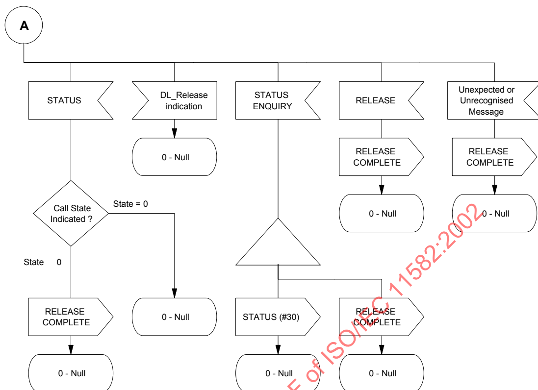
Figure 9 — Connection oriented Protocol Control SDL (Sheet 2 of 10)
