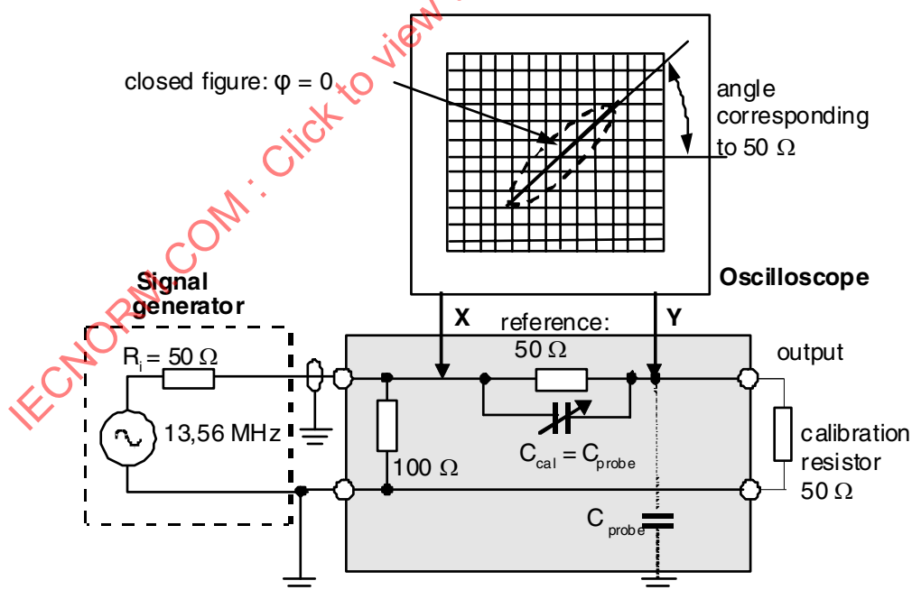
Figure B.1 — Calibration set-up (Step 1)
