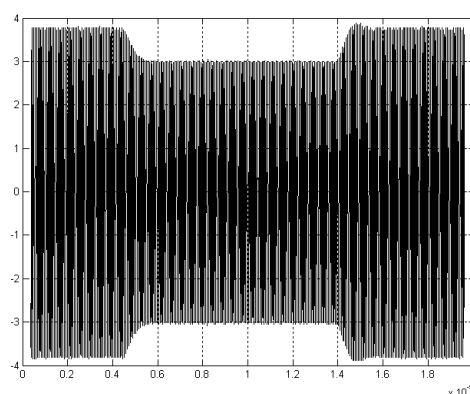
Figure E.2 — Modulation pulse
