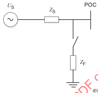
Figure 9 – Layout of grid with symmetrical fault
