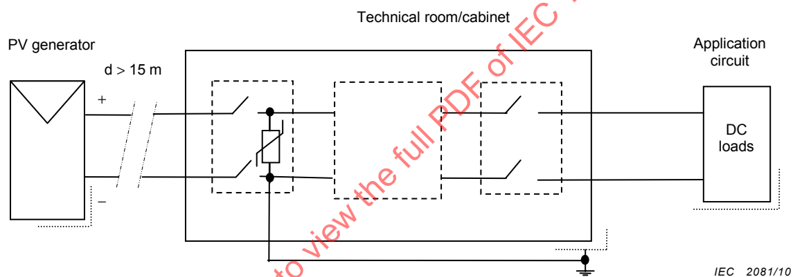
Figure 3 – Configuration G – PV alone IES P < 500 \text{ W} – without inverter – d > 15 \text{ m}
