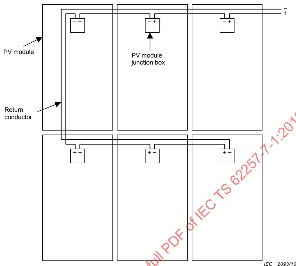
Figure 15 – PV string wiring with minimum loop area
