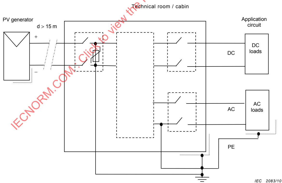
Figure 5 – Configuration H – PV alone IES P < 500 \text{ W} – with inverter – d > 15 \text{ m}
