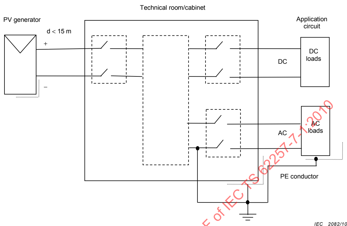
Figure 4 – Configuration B – PV alone IES P < 500 \text{ W} – with inverter – d < 15 \text{ m}
