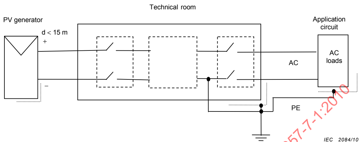
Figure 6 – Configuration C and E – PV alone IES or CES – P < 500 \text{ W} – with inverter – d < 15 \text{ m}
