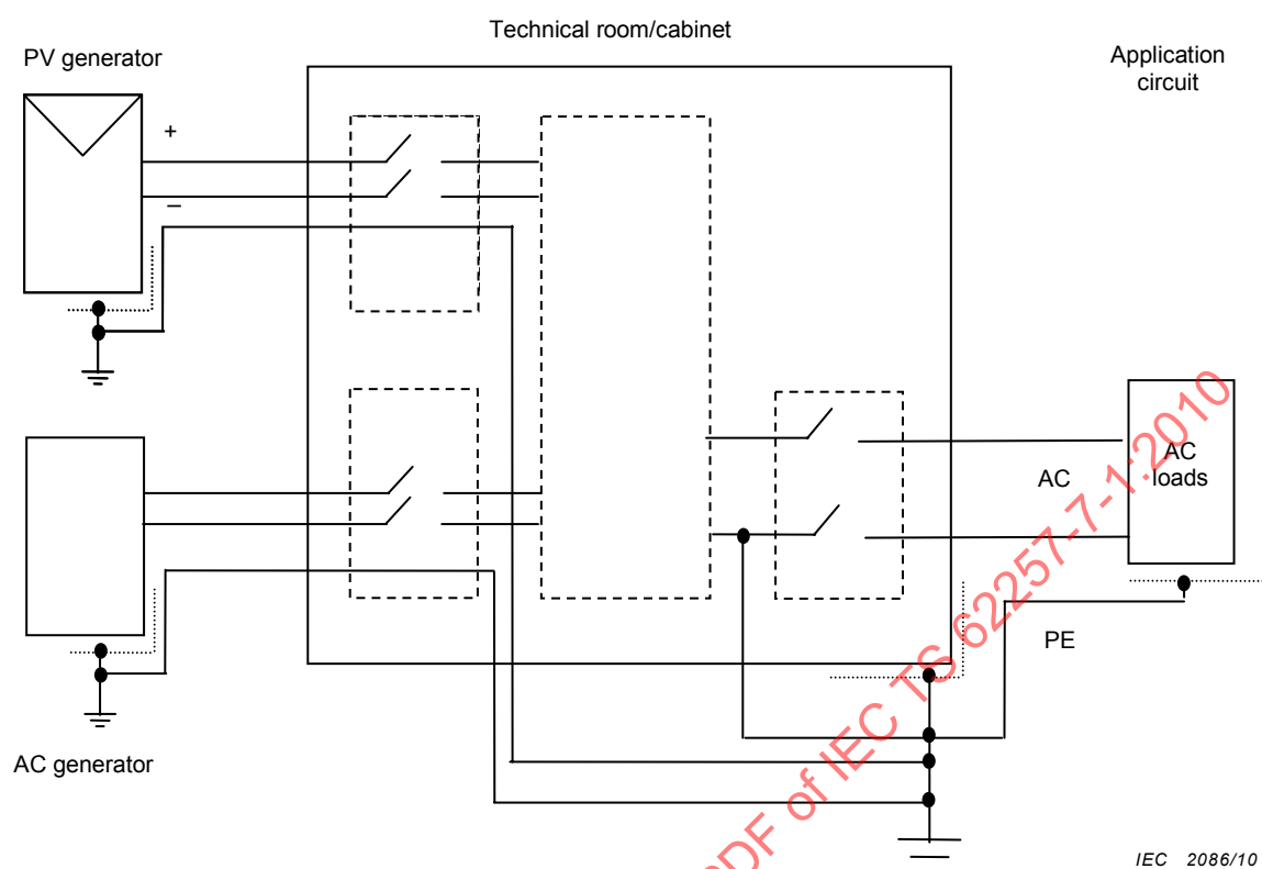
Figure 8 – Configuration D and F – Hybrid IES or CES – PV generator + inverter and other generator – d < 15 m
