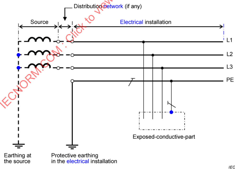
Figure B.12 – TT system 3-phase, 3-wire with earthed protective conductor and no distributed neutral conductor throughout the distribution system
