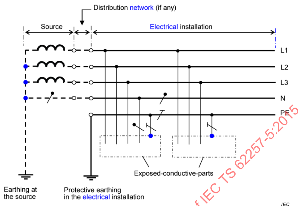
Figure B.11 – TT system 3-phase, 4-wire with earthed protective conductor and neutral conductor throughout the distribution system
