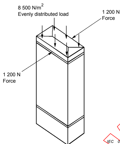
Figure 102 – Diagram of test to verify the resistance to static load
