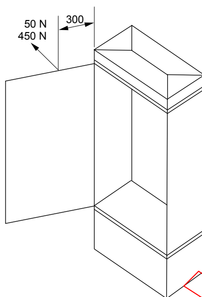
Figure 106 – Diagram of test to verify the mechanical strength of doors
