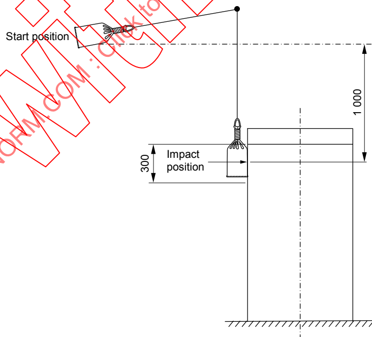
Figure 104b – Diagram of test to verify the resistance to shock load of a ground-mounted ASSEMBLY without embedded base
