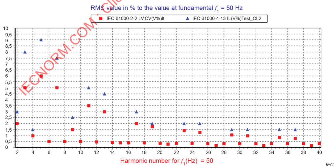
Figure 11 – LVAC voltage compatibility and immunity levels
