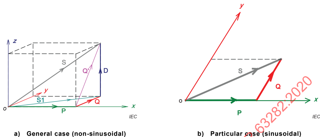
Figure C.2 – Representation of electric powers in AC system
