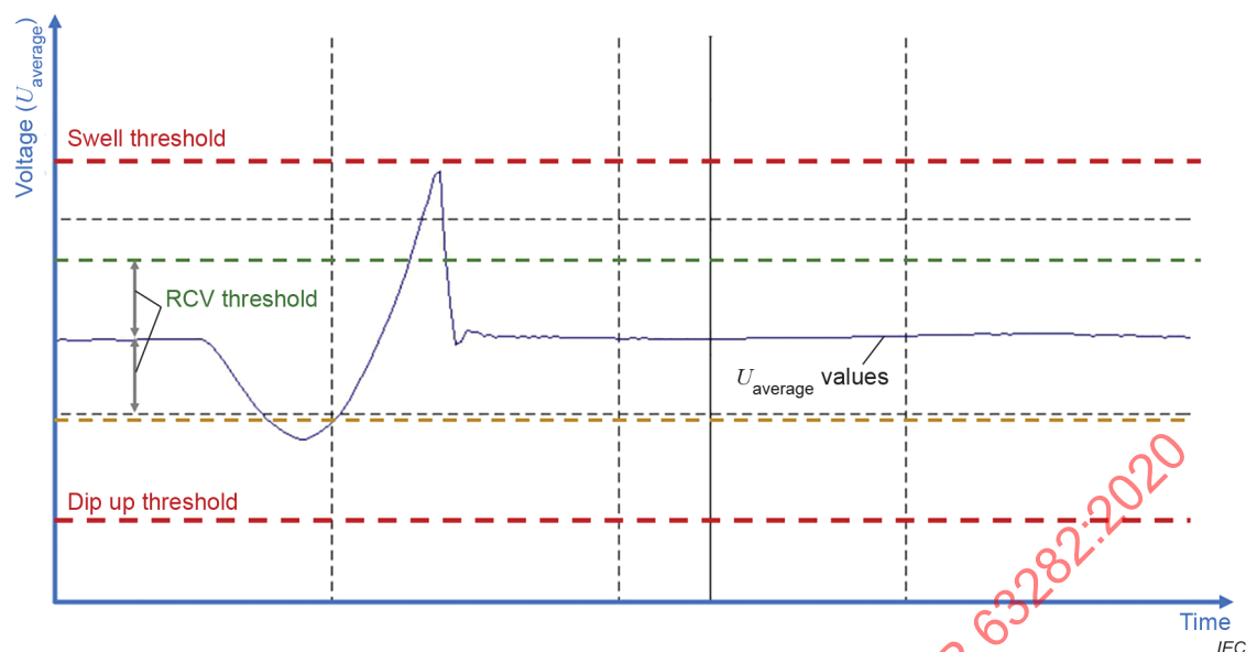
Figure 7 – RVC event: example of a change in average voltage that results in an RVC event
