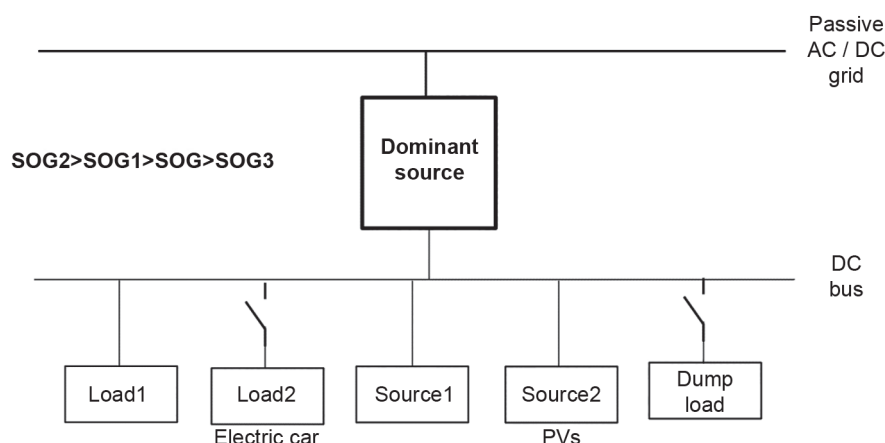
Figure F.5 – Distribution system with more than one load and source in overloaded mode
