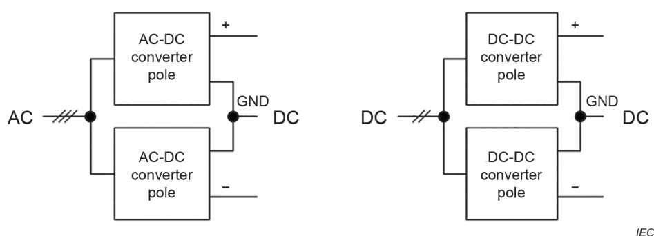
Figure 9 – A schematic of a bipolar system (the CIGRE B4 DC test system)
