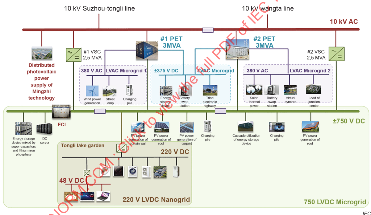
Figure D.1 – Architecture of the district LVDC system in Tongli
