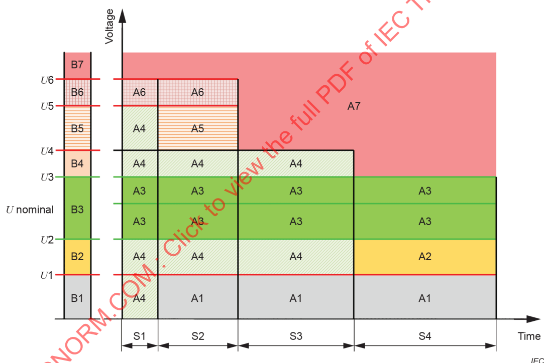
Figure 3 – DC Voltage areas for safe interoperability
