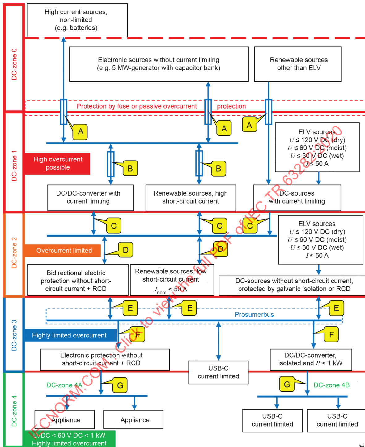
Figure E.2 – Overview of DC-zones for DC system
