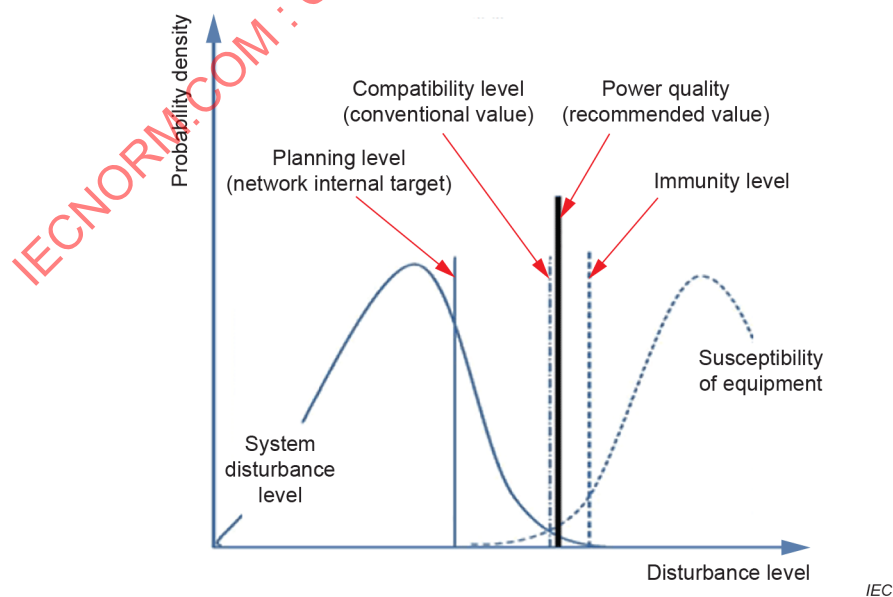
Figure 10 – Relation between disturbance levels (schematic significance only)
