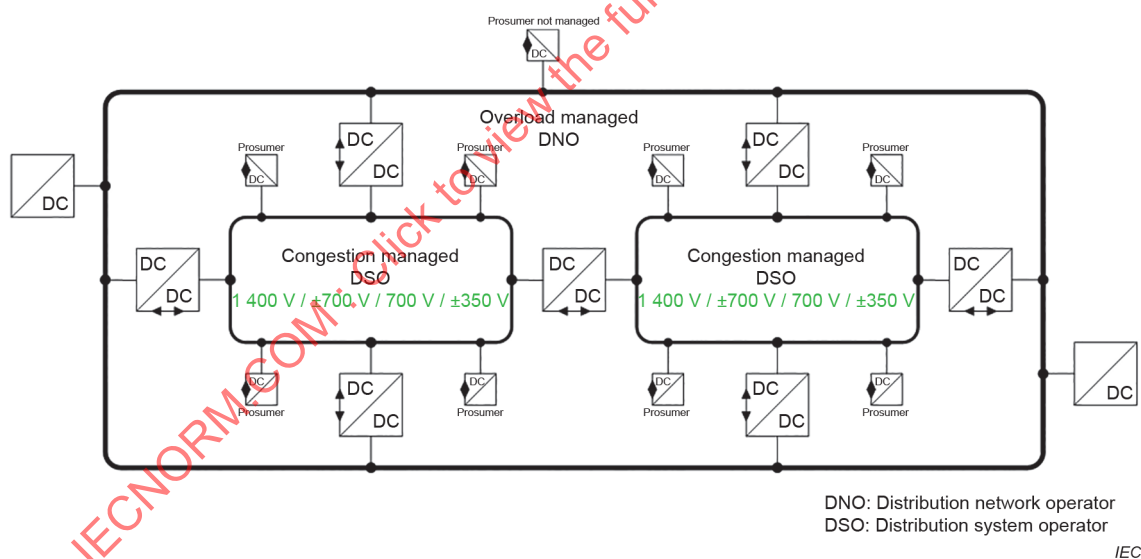
Figure F.1 – Active DC distribution system
