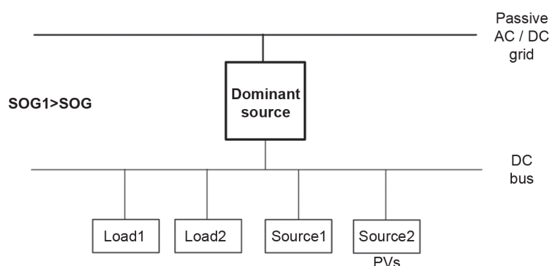
Figure F.3 – DC distribution system with more than one load and a source and increasing source power
