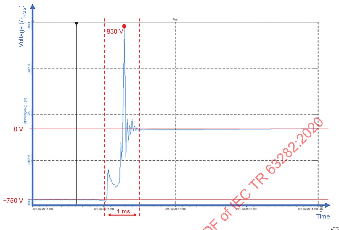
Figure 8 – Example of voltage surge
