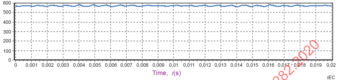
Figure C.4 – Ripples
