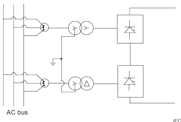
a) Two-winding converter transformer connection
