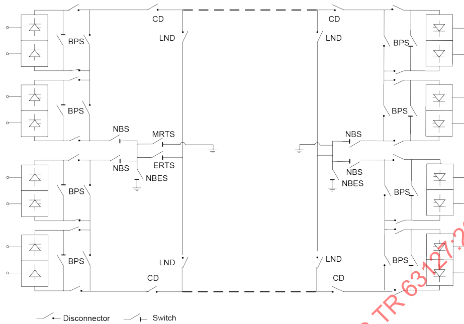
a) Sketch map with two twelve-pulse valve converters in series connection per pole
