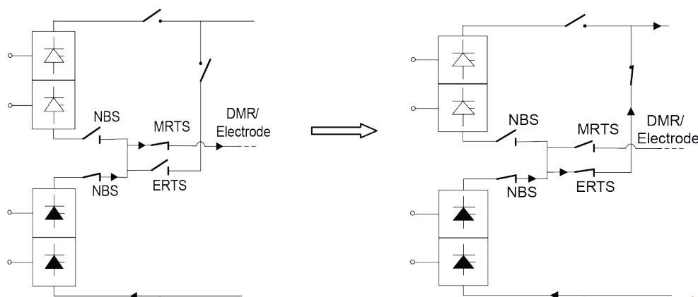
Figure 11 – Current transfer path of the MRTS
