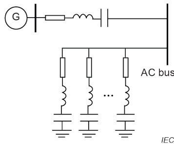
Figure 5 – Structure of equivalent network for low order harmonic resonance study
