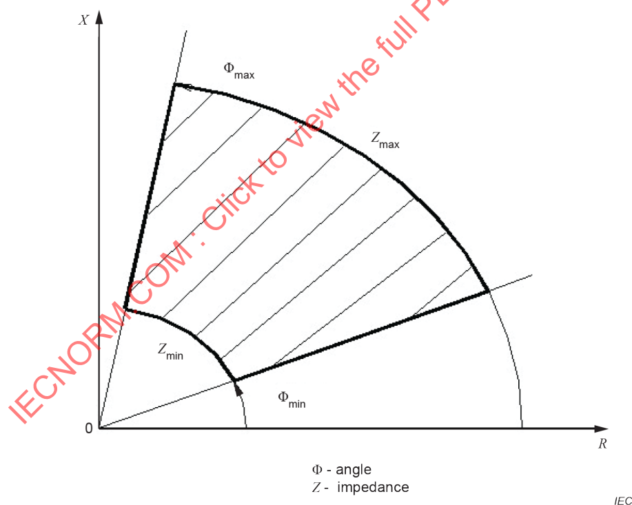
Figure 3 – Sector diagram of system harmonic impedance
