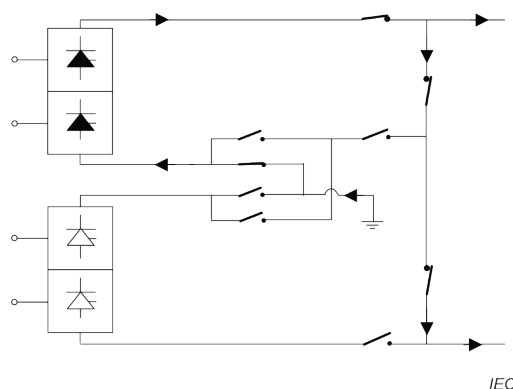
Figure 9 – Schematic diagram of pole line parallel connection
