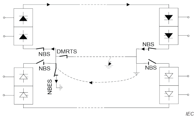
b) Current transfer path of DMR after NBES disconnecting grounding fault
