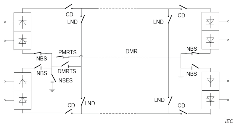
c) Sketch map with dedicated metallic return line as return path
