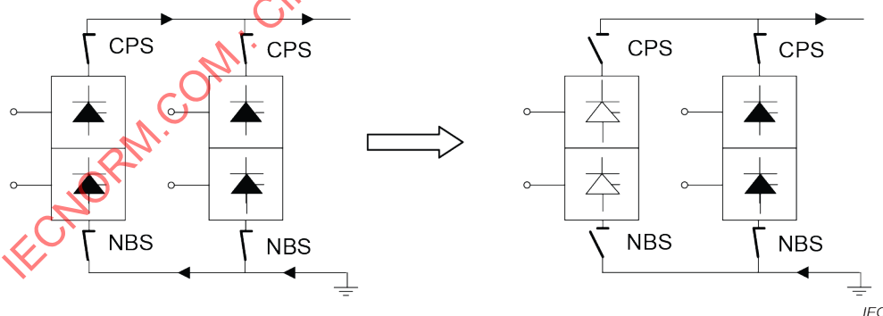
Figure 16 – Converter paralleling switches
