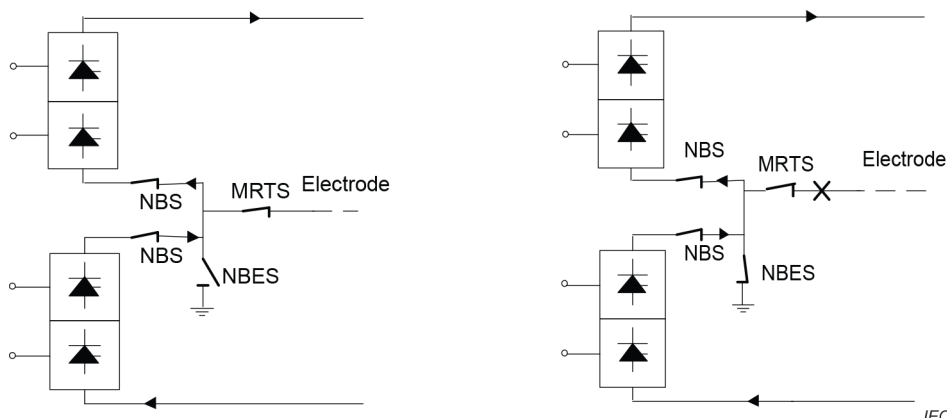
Figure 13 – Connection and function of the NBES
