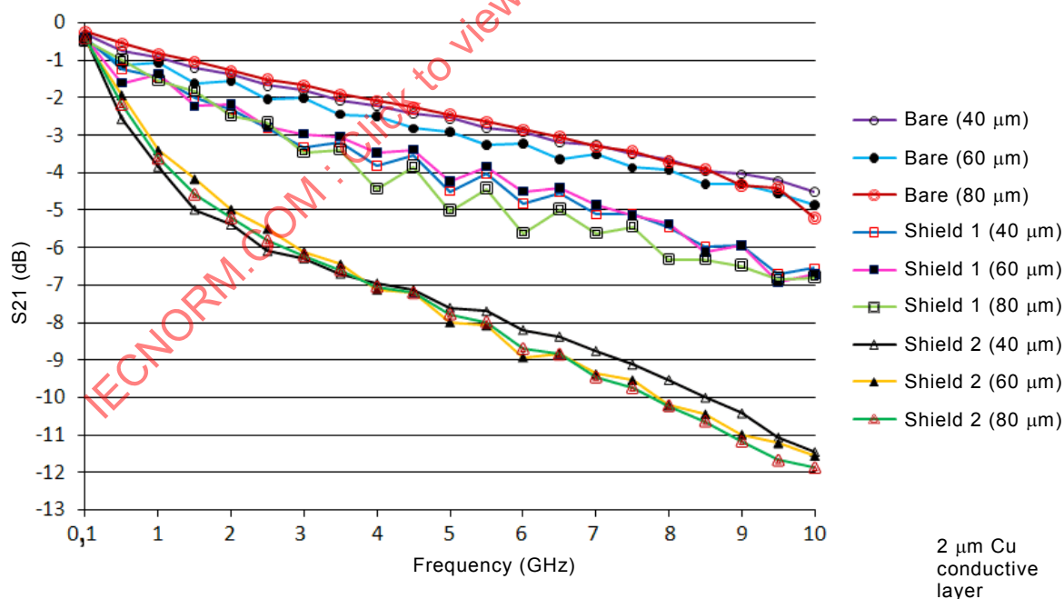
Figure 9 – Signal loss variation according to the Cu signal line width
