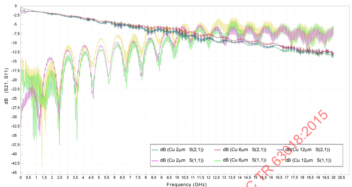
Figure 8 – Signal loss variation according to the Cu conductive layer thickness
