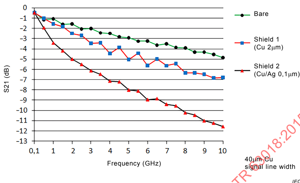
Figure 7 – Signal loss value of the bare and shield FPCB
