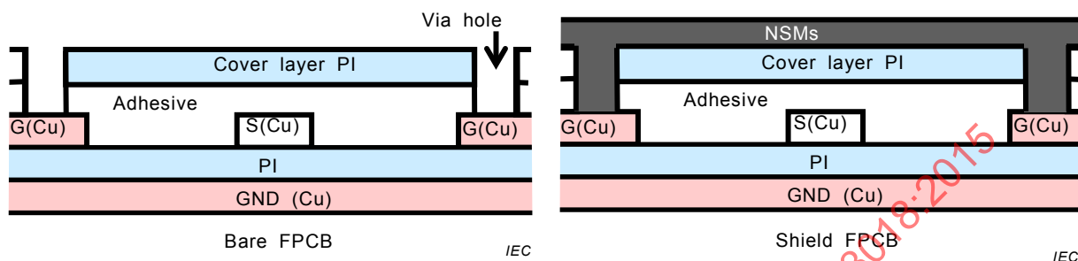
Figure 10 a – <FPCB of micro strip line structure>
