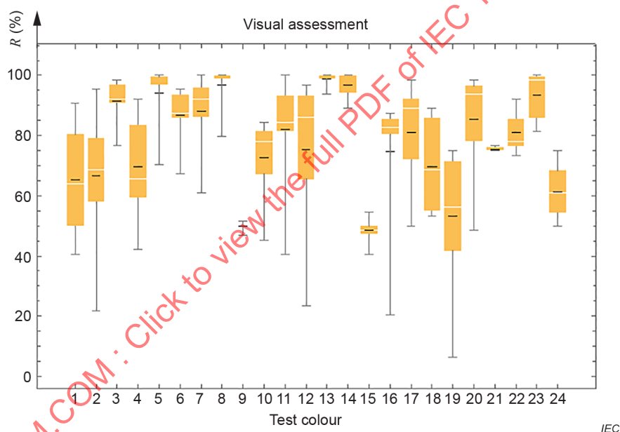
Figure 16 – Pattern dependency
