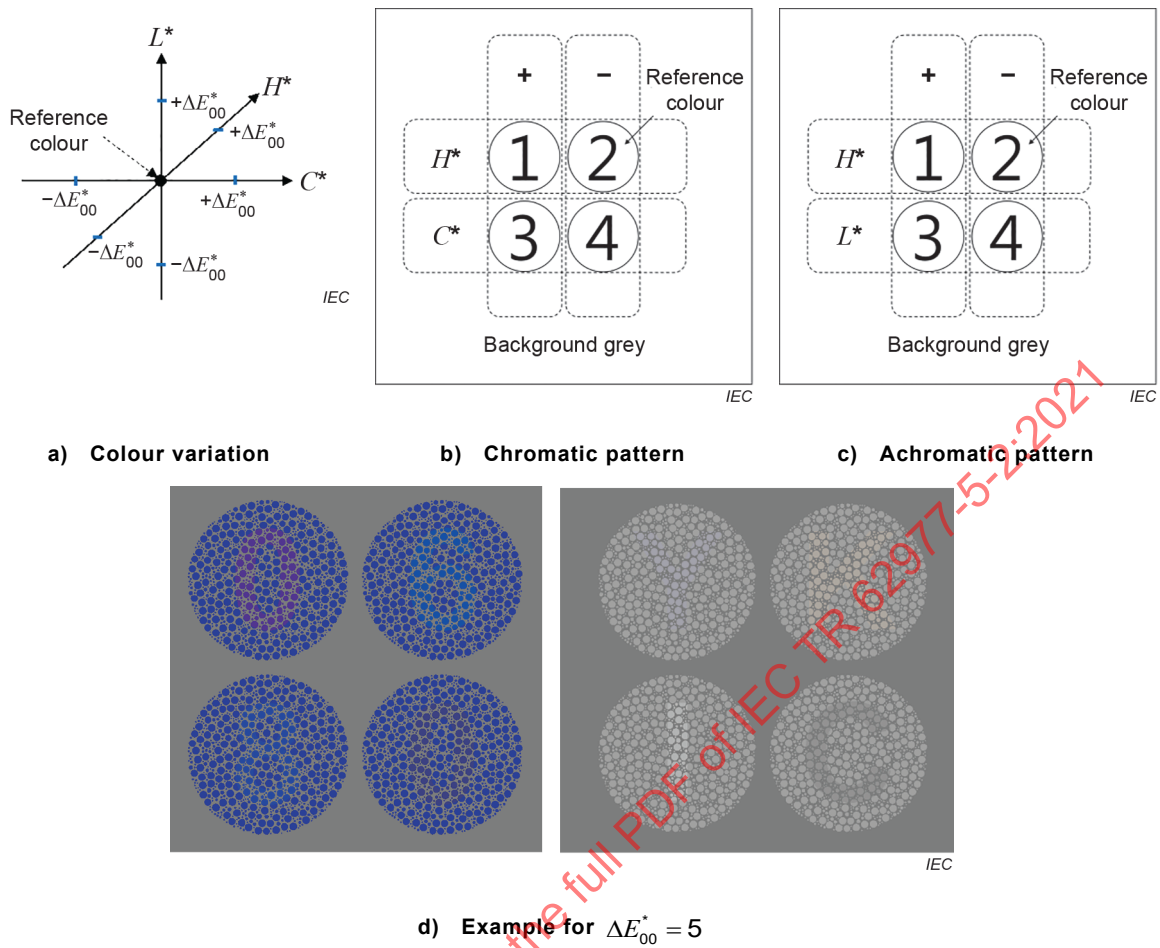
Figure 5 – Colour assignment of test pattern
