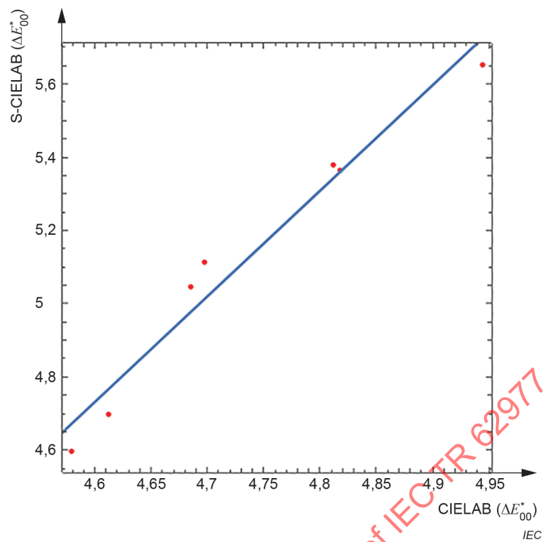
Figure 14 – Correlation between physical measures and S-CIELAB results
