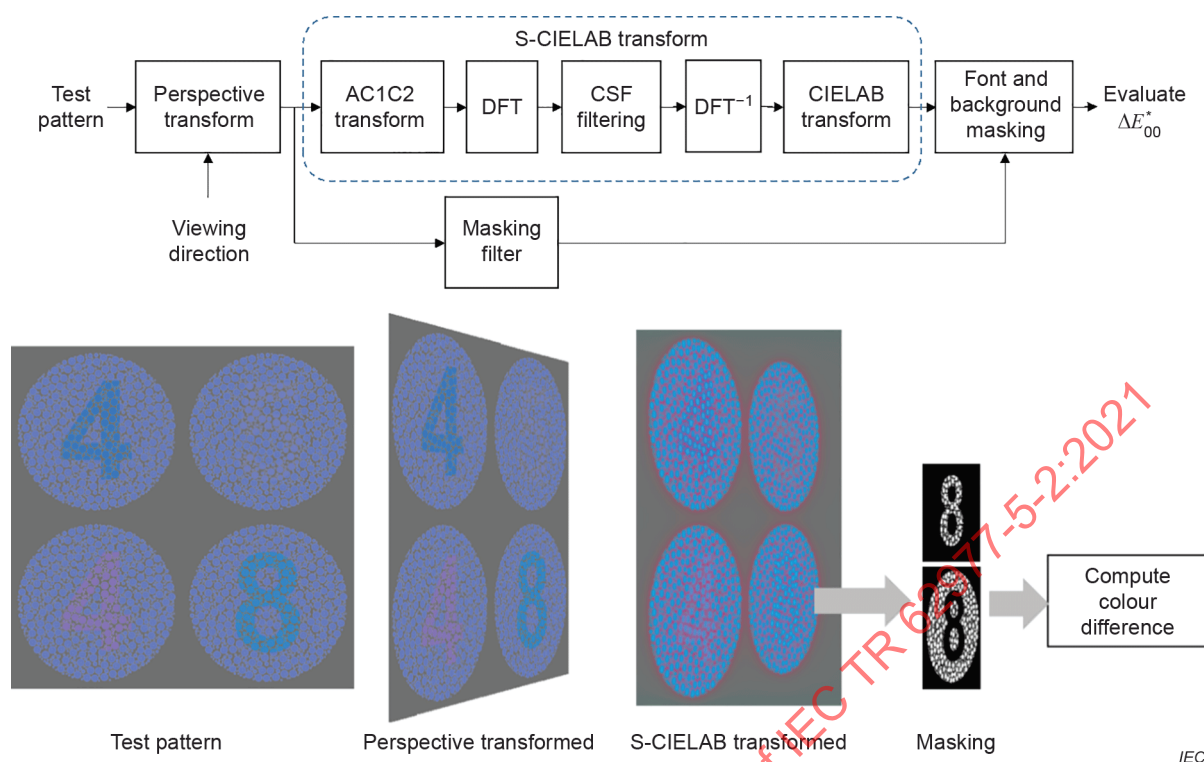
Figure 11 – Process of S-CIELAB transformation
