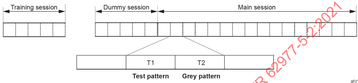
Figure 8 – Assessment procedure
