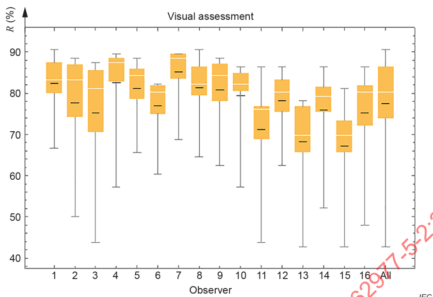
Figure 17 – Observer dependency
