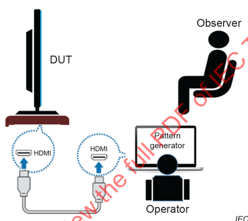
Figure 6 – Test environment
