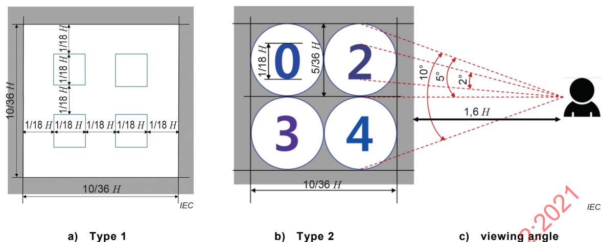
Figure 4 – Pattern structures
