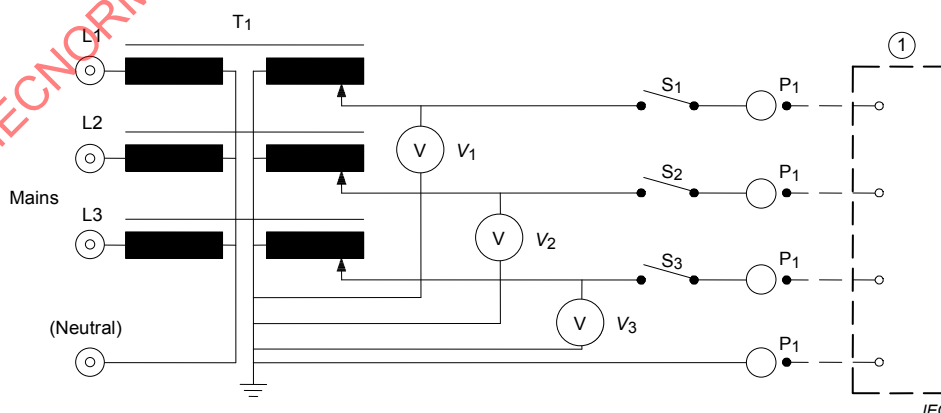
Figure D.3 – Measuring supply circuit for polyphase ME EQUIPMENT specified for connection to a polyphase SUPPLY MAINS
