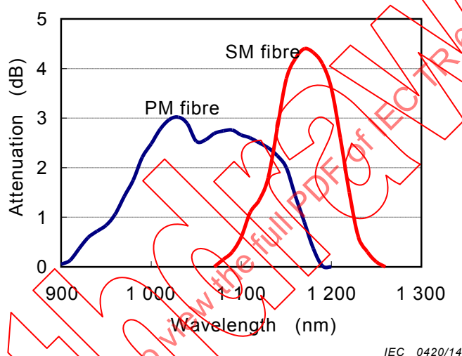
Figure A. 1 – Cut-off wavelength profiles of PM fibre and SM fibre
