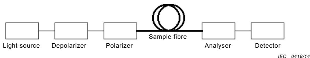
Figure 3 – Example of test apparatus for polarization crosstalk measurement (power ratio method)
