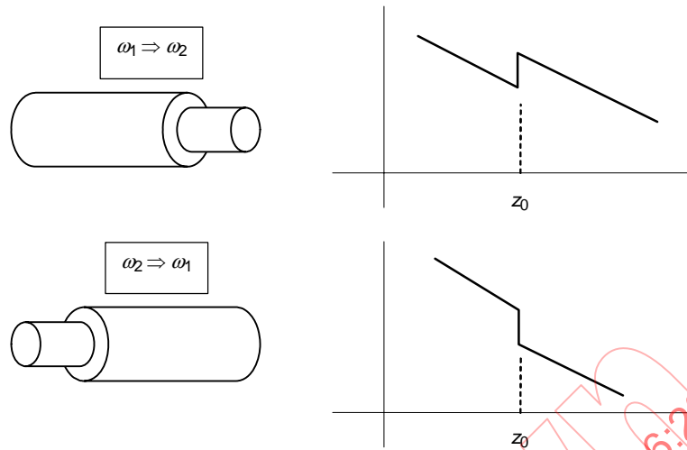
Figure 2 – OTDR traces for fibres with different MFD
