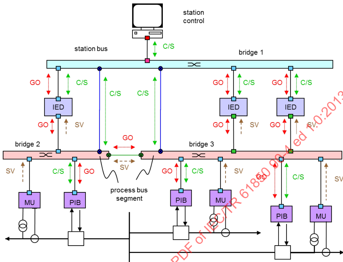
Figure 55 – Traffic patterns
