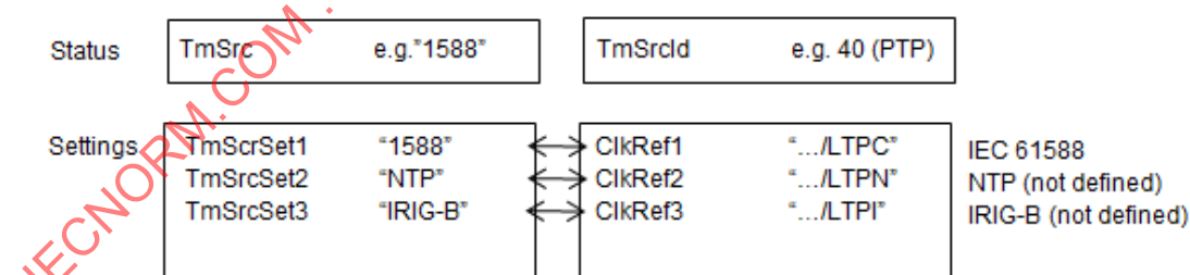
Figure 83 – Usage of clock references
