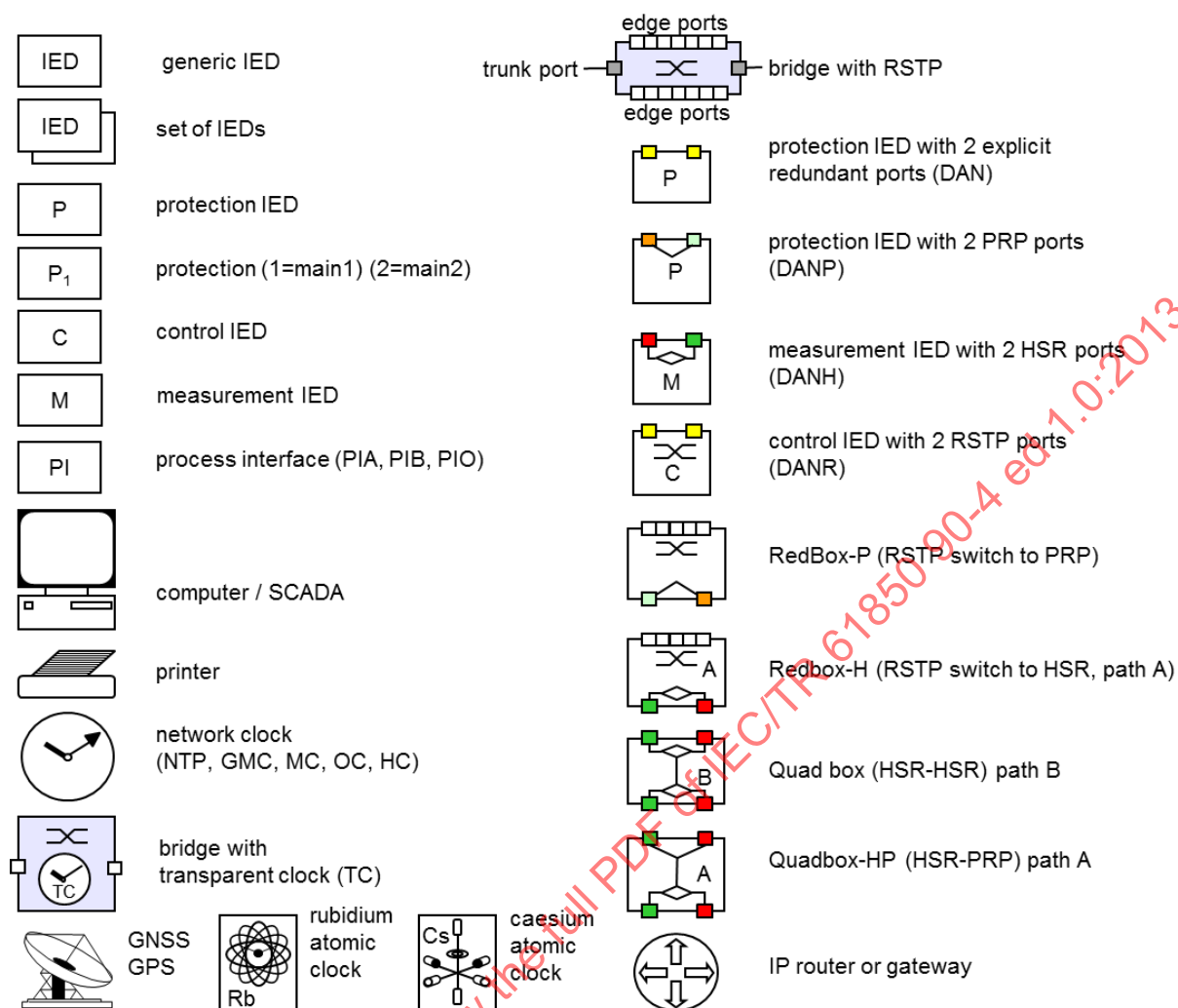
Figure 1 – Network symbols
