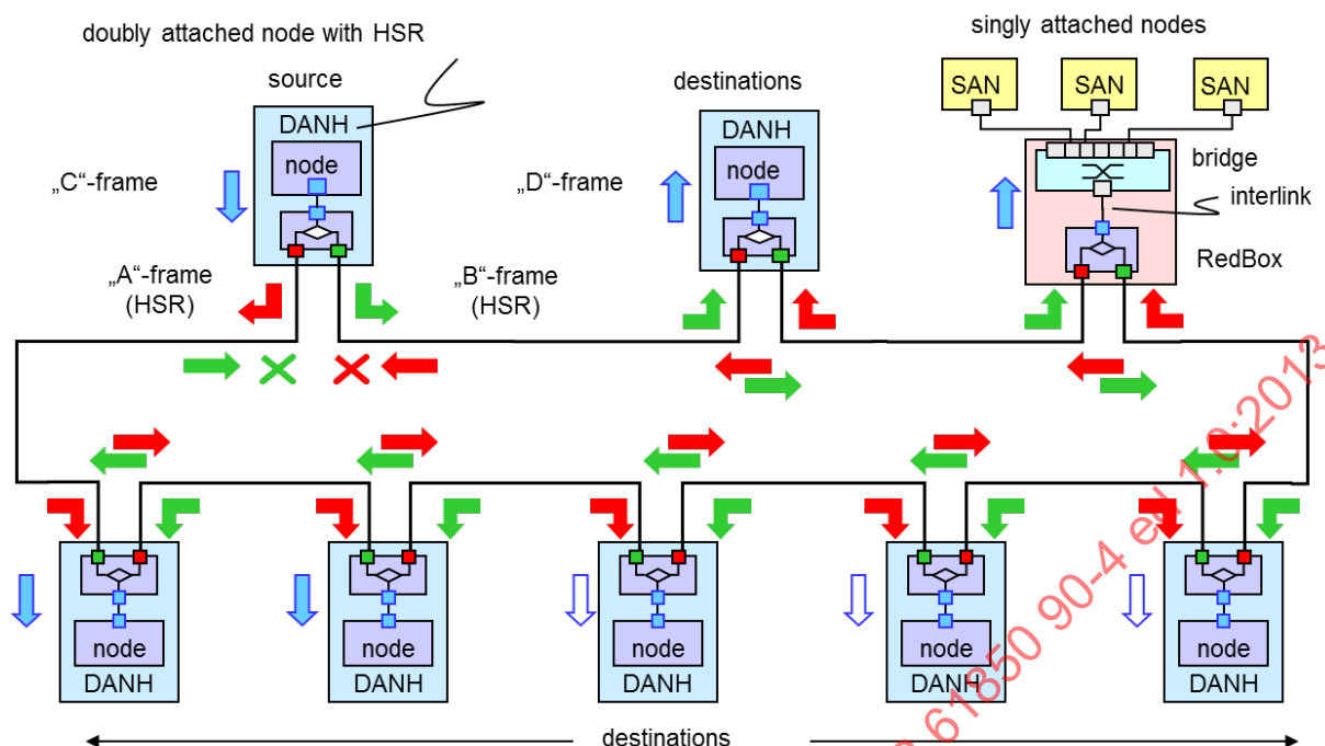
Figure 21 – HSR principle
