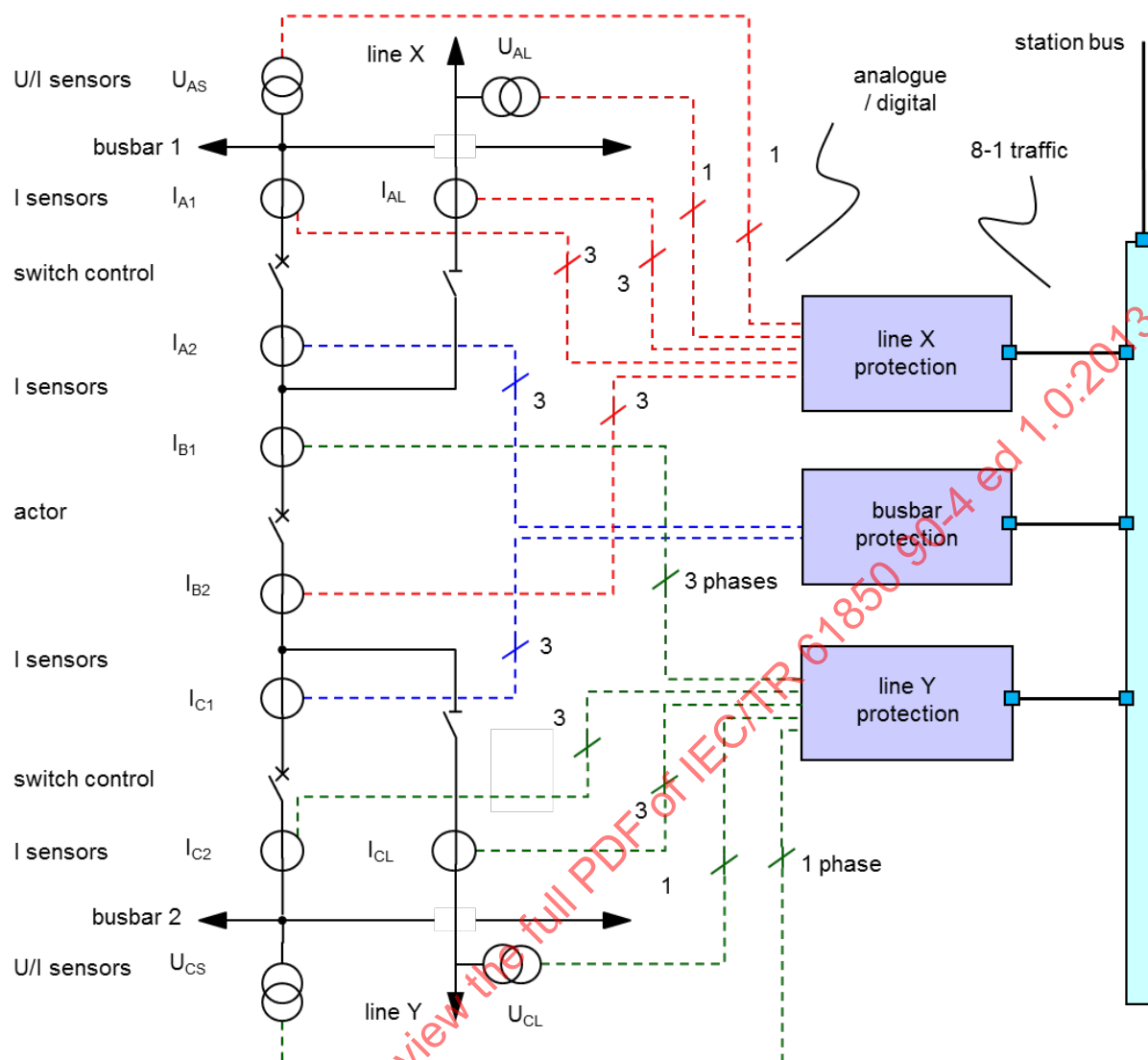
Figure 39 – 1 ½ CB diameter with conventional, non-redundant attachment
