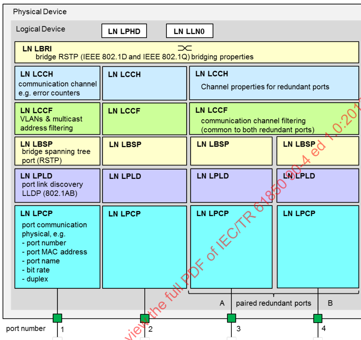
Figure 75 – Multiport device model
