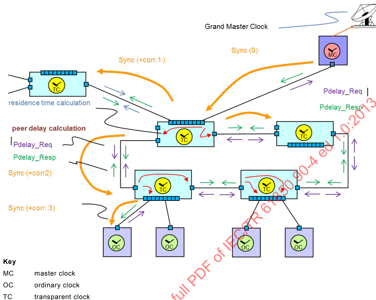
Figure 67 – PTP elements
