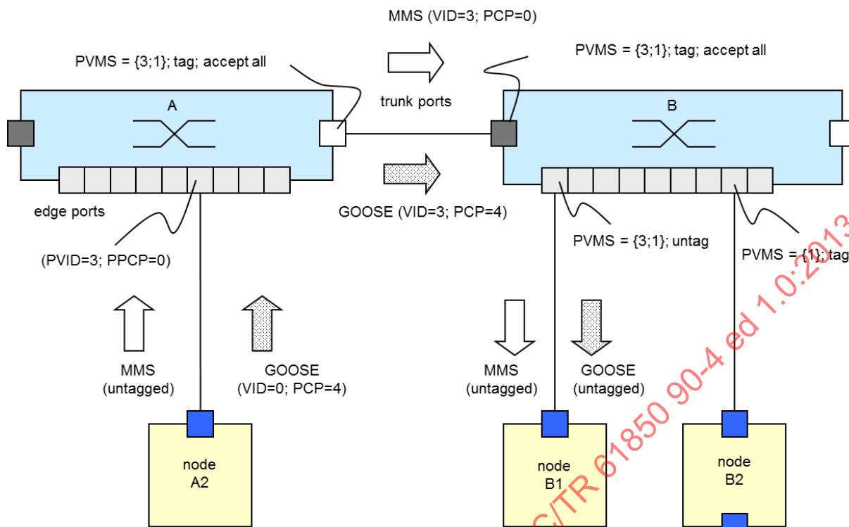
Figure 57 – Bridges with correct VLAN configuration
