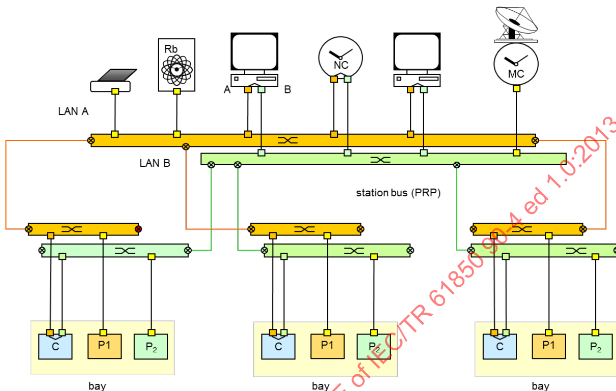
Figure 26 – Station bus as dual star with PRP
