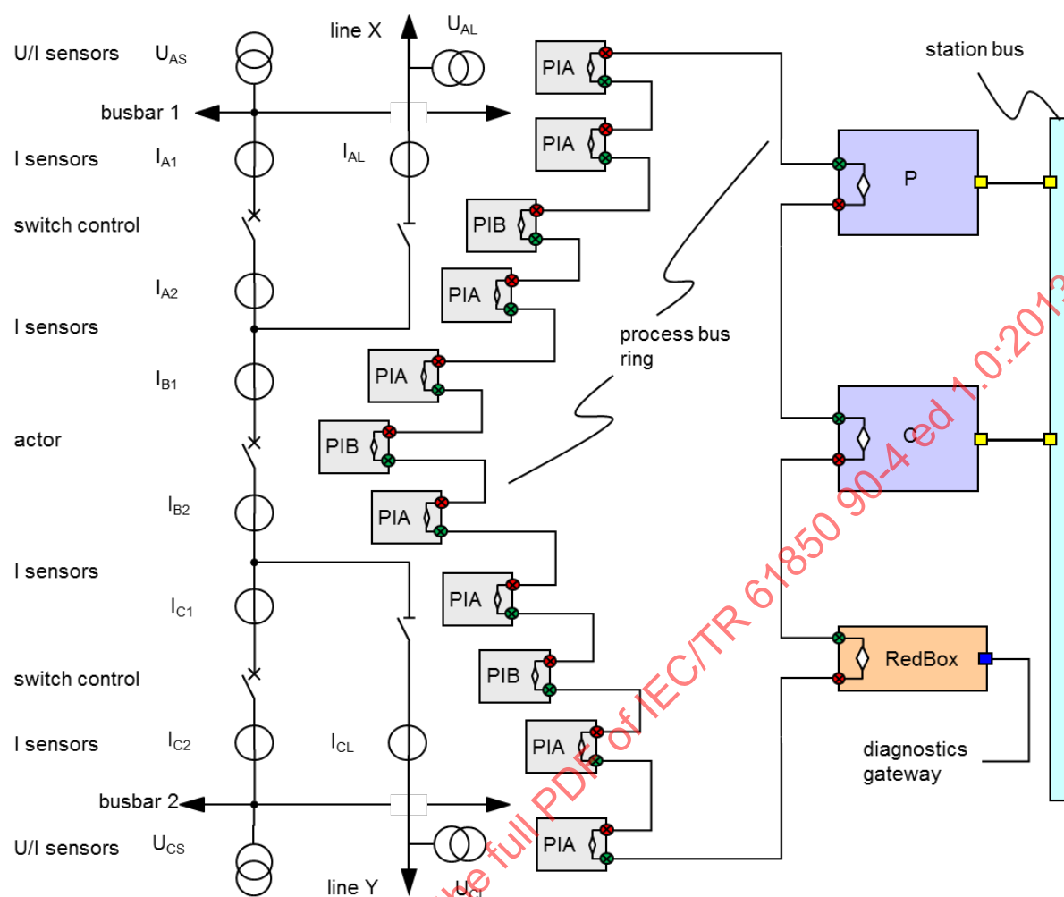
Figure 47 – Process bus as ring of HSR nodes
