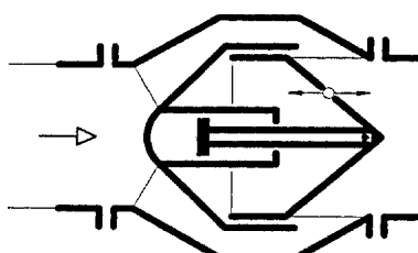
Figure 10f – Needle valve Vanne pointeau
