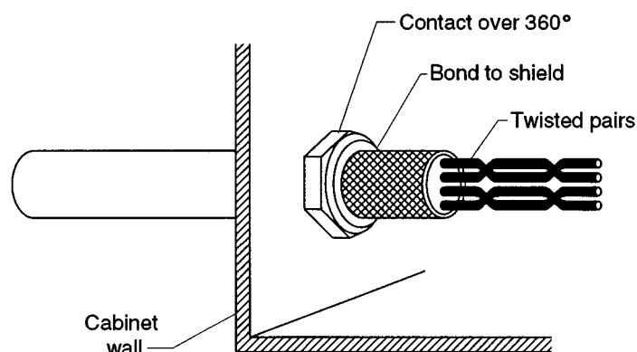
Figure 15 – Example of optimal bonding of a shielded cable to the enclosure by a compression fitting providing a 360-degree bond
