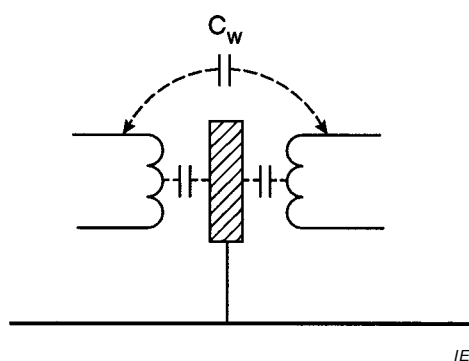
Figure 28 – Limitations in the effectiveness of an isolation transformer
