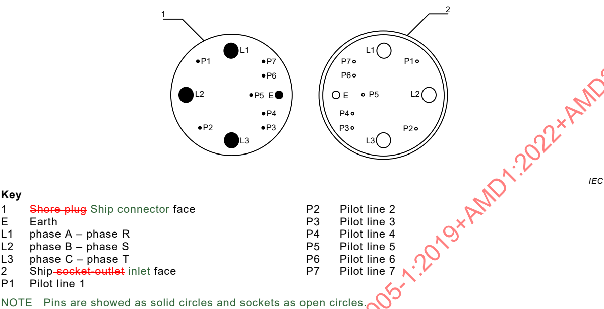
Figure B.3 – Three-phase plug ship connector and socket-outlet ship inlet contact assignment
