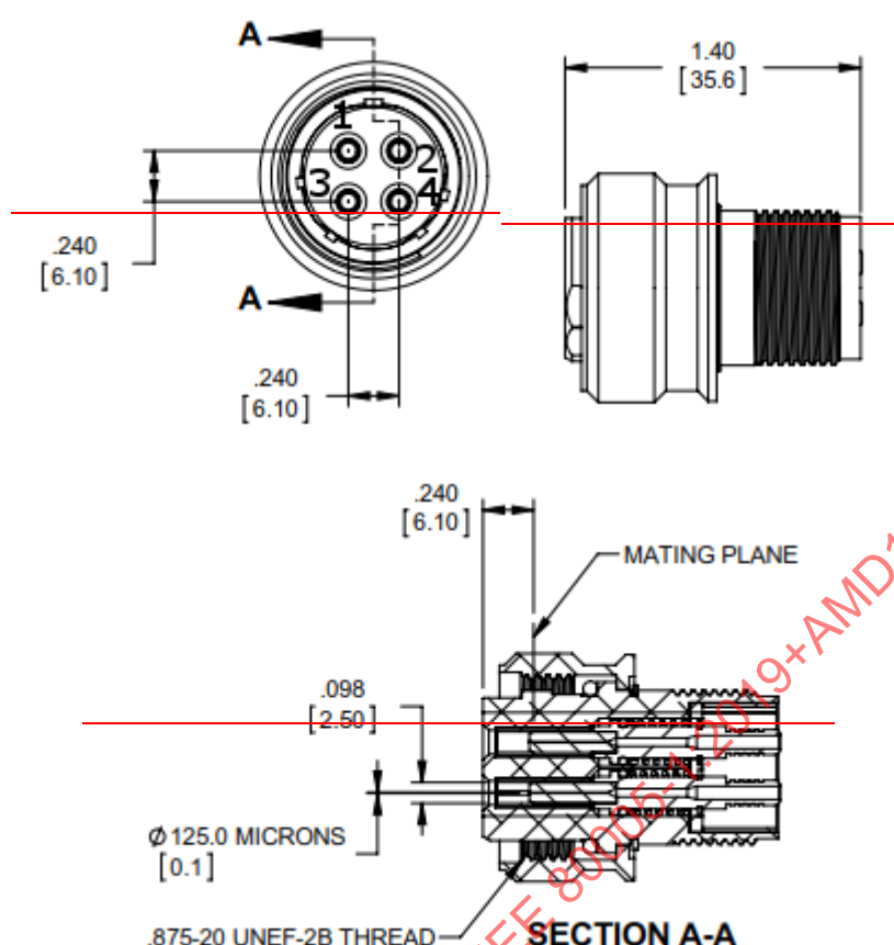
Figure 5 — Fibre optic plug
