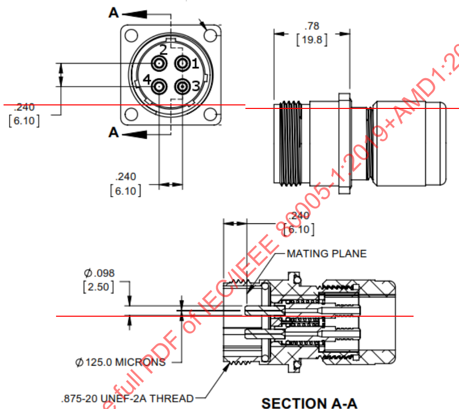
Figure 4 — Fibre-optic socket outlet
