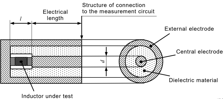
Figure 2 – Fixture A
