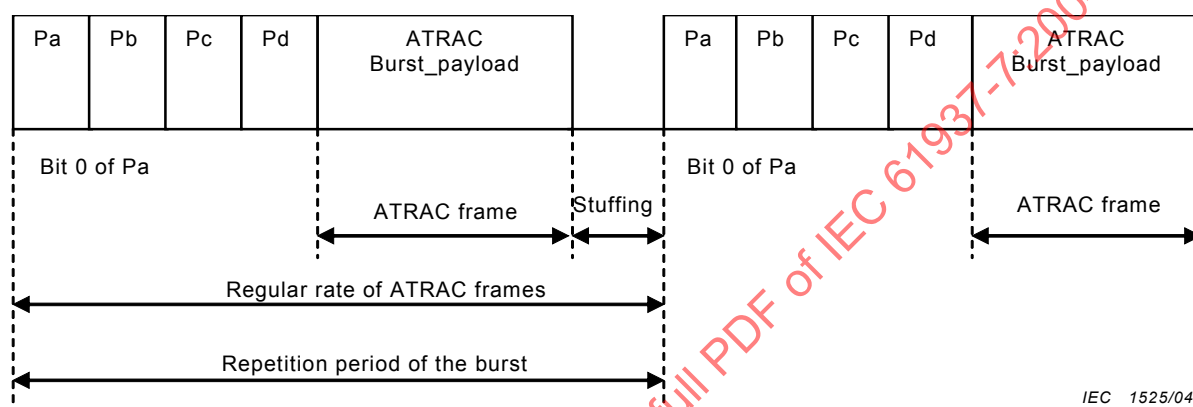
Figure 1 – ATRAC data-burst
