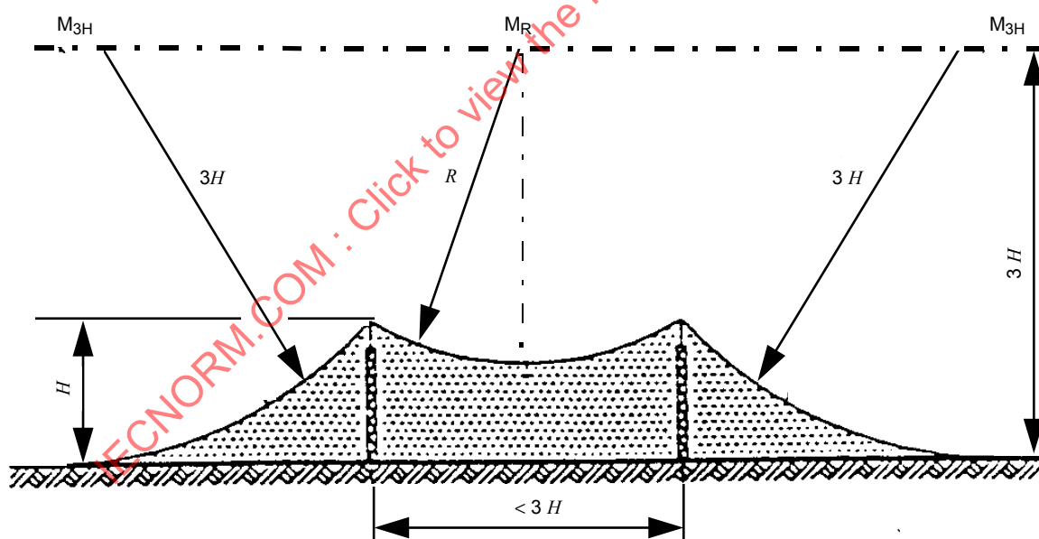
Figure E.4 – Two lightning rods
