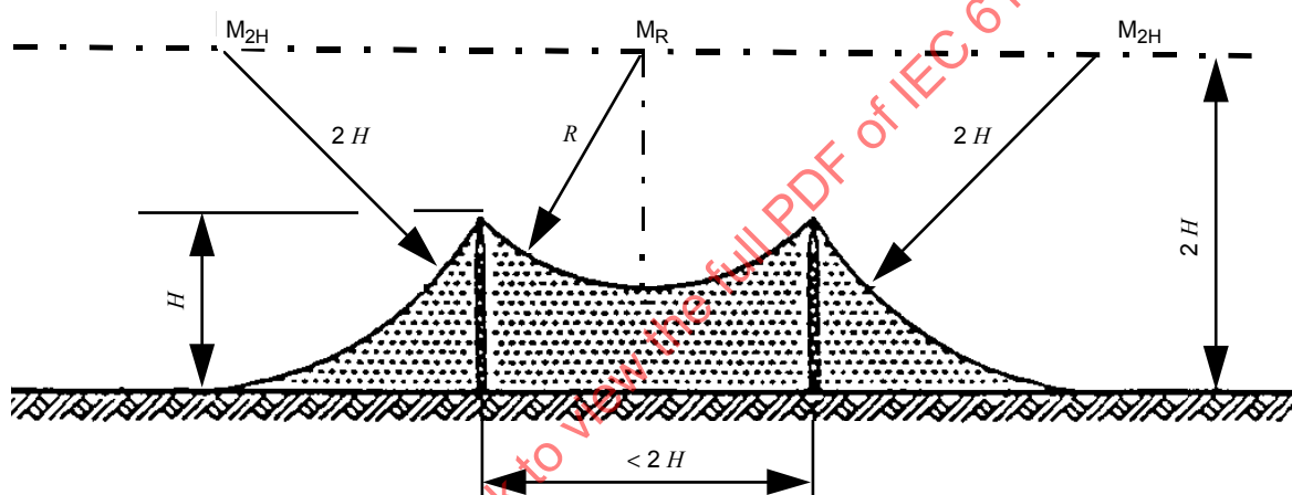
Figure E.2 – Two shield wires
