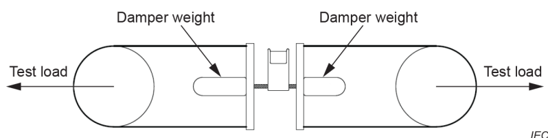
Figure 2 – Test arrangement for attachment of weights to messenger cable test
