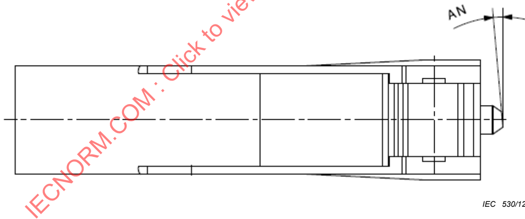
Figure 3 – Top view (APC)
