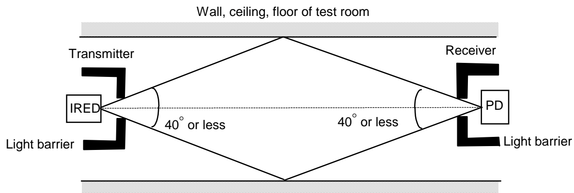
Figure 2 – Location for measuring
