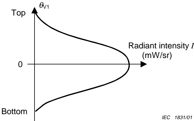
Figure 8b – Vertical directivity
