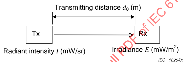
Figure 3 – Transmitting distance
