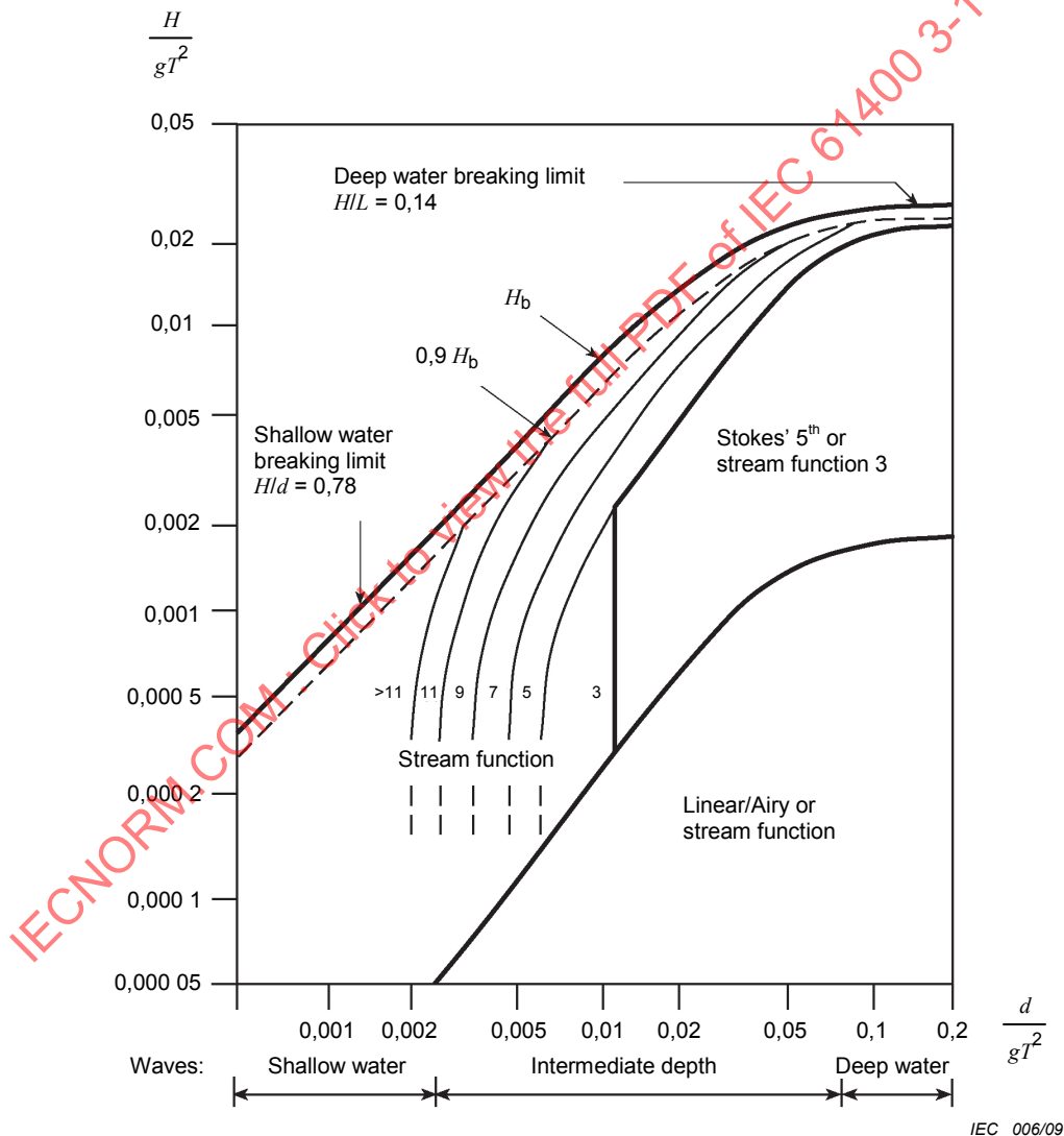
Figure C.1 – Regular wave theory selection diagram
