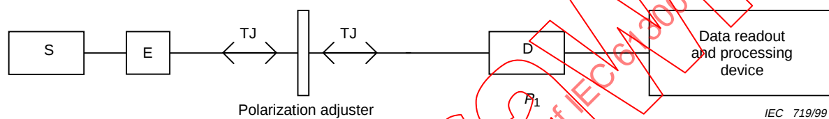
Figure 3c – Cutback – Step 3
