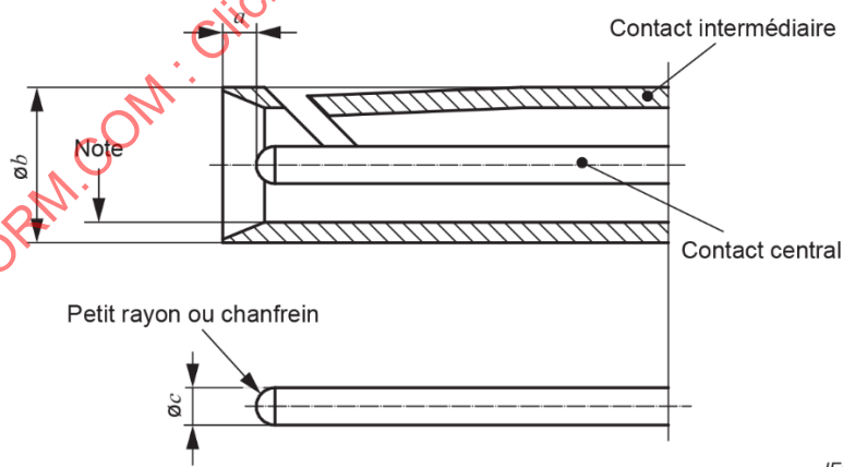
Figure 4 – Contact femelle coaxial
