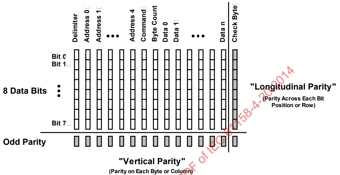
Figure 8 – Two dimensional parity detection
