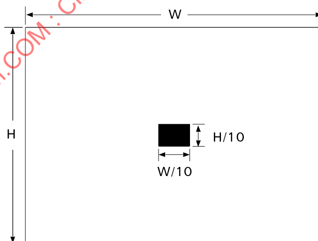
Figure 17 – Specification of the test chart for measurement of localized flare (average picture level = 99 %)
