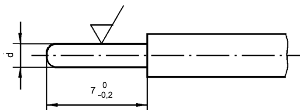
Figure 5 – Gauge
