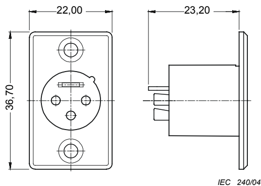
Figure 7 – Taille 1M
