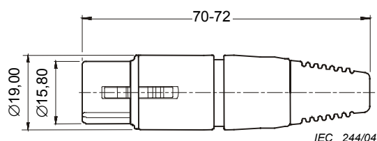
Figure 11 – Female straight connector
