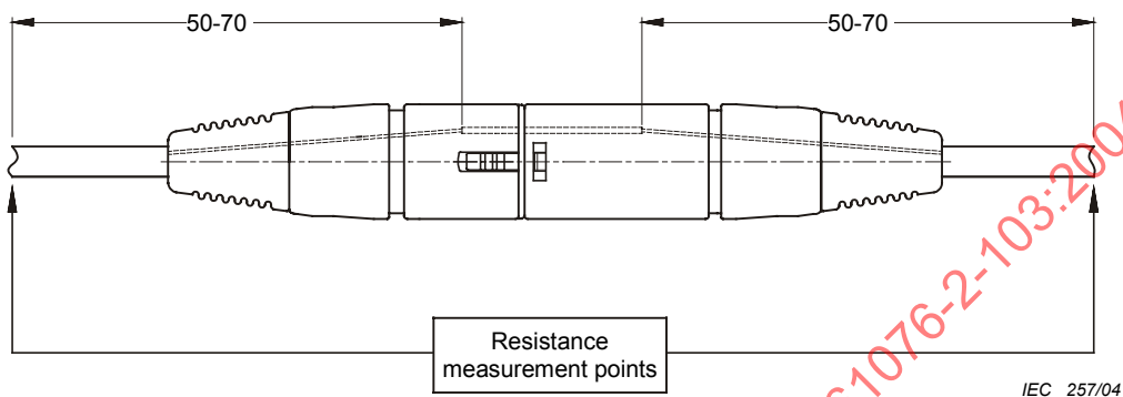
Figure 24 – Mating of free connectors
