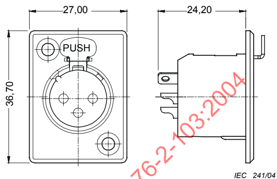
Figure 8 – Taille 1F
