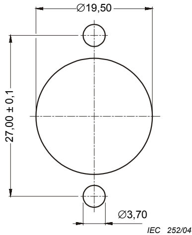
Figure 19 – Variante 1M
