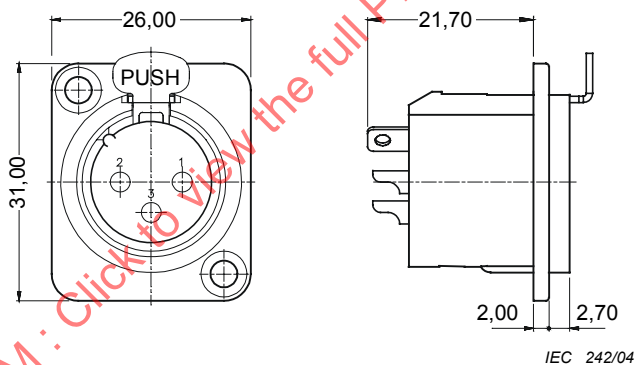
Figure 9 – Taille 2
