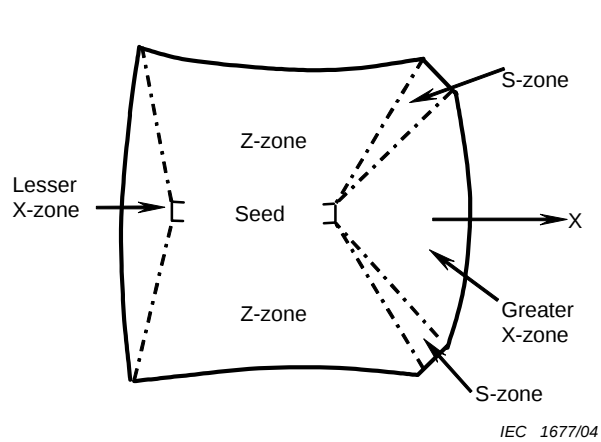
Figure 1a – Section \perp to Y-axis
