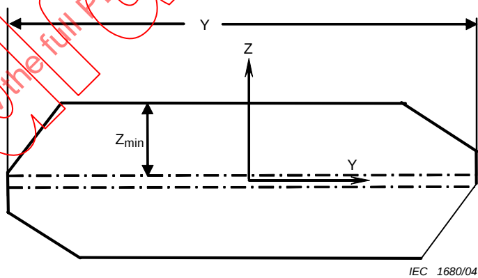
Figure 1d – Illustration of dimension Zmin
