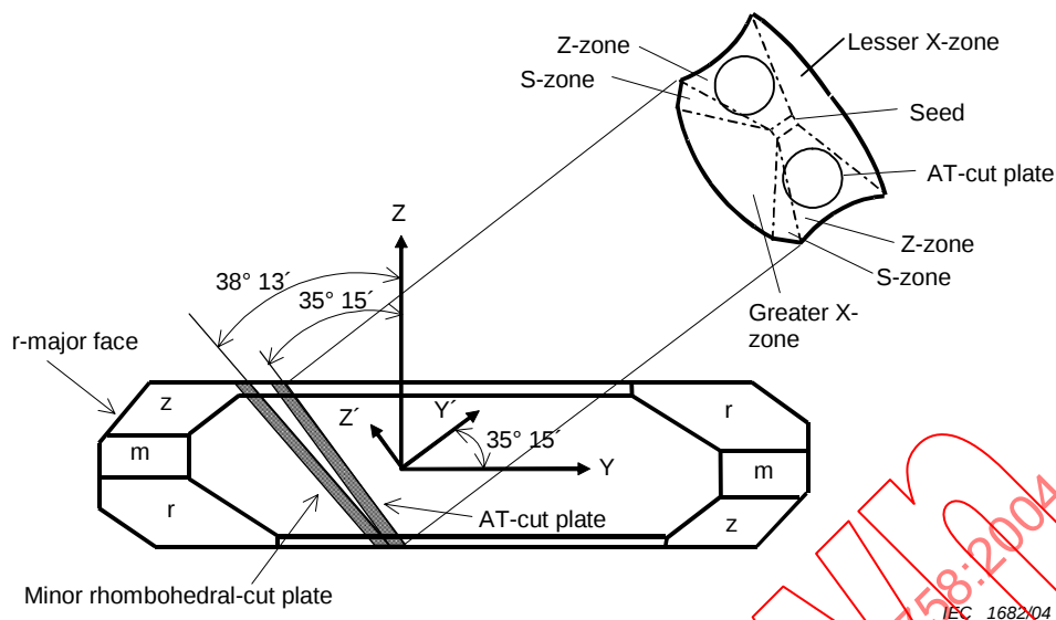
Figure 3a – Location of AT-cut plates in right-handed synthetic quartz with 0° orientation
