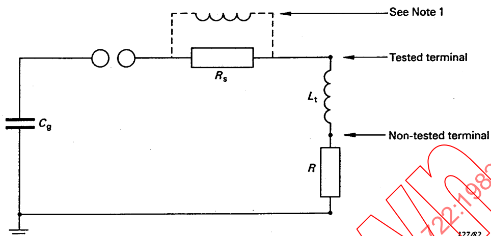
FIG. 8. — Resistance earthing of low impedance windings.
