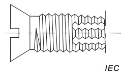
Figure 7 – Thread-cutting screw
