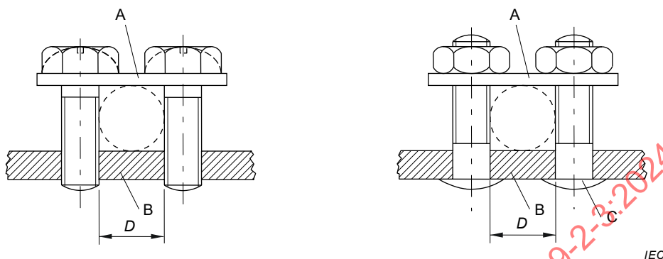
Figure 2 – Screw head terminals and stud terminals
