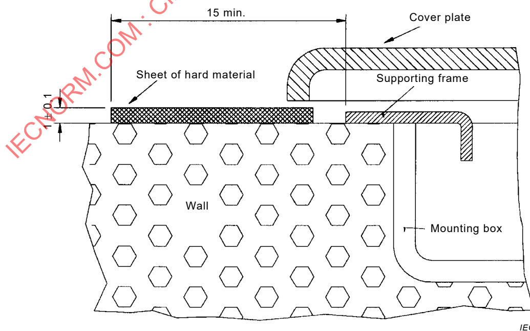
Figure 13 – Arrangement for test on cover-plates
