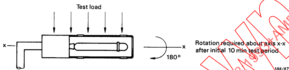
Detail b) – Initial test position
