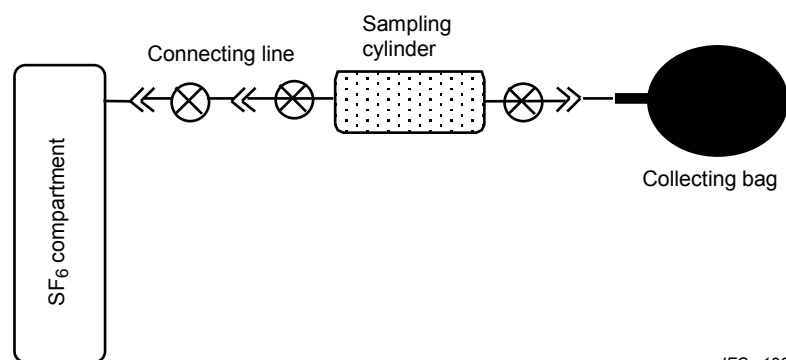
Figure B.2 – SF 6 gas sampling set-up: purging
