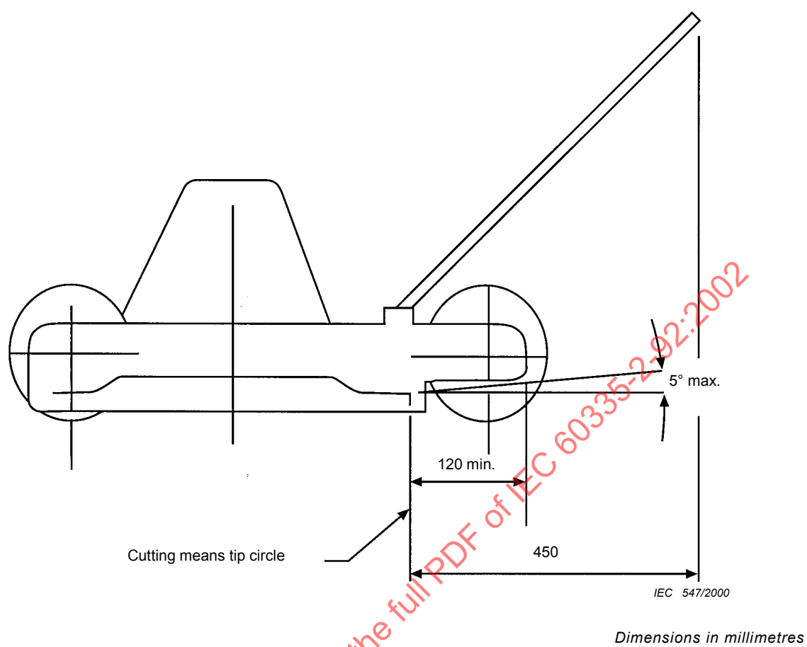
Figure 101 – Safety distances – Rotary appliances
